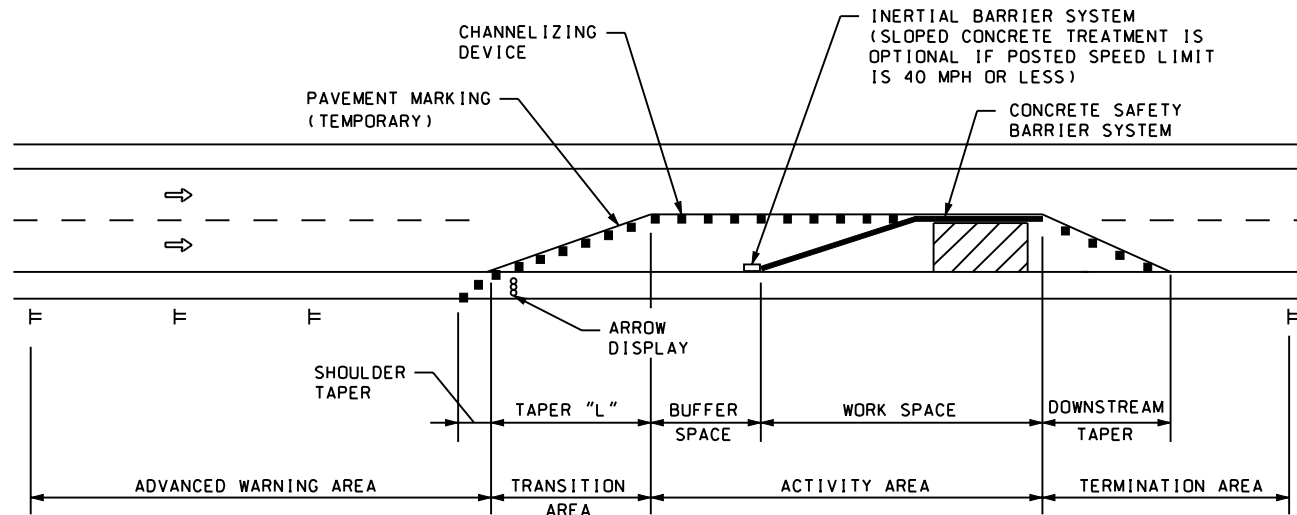
TYPICAL WORK ZONE COMPONENTS
