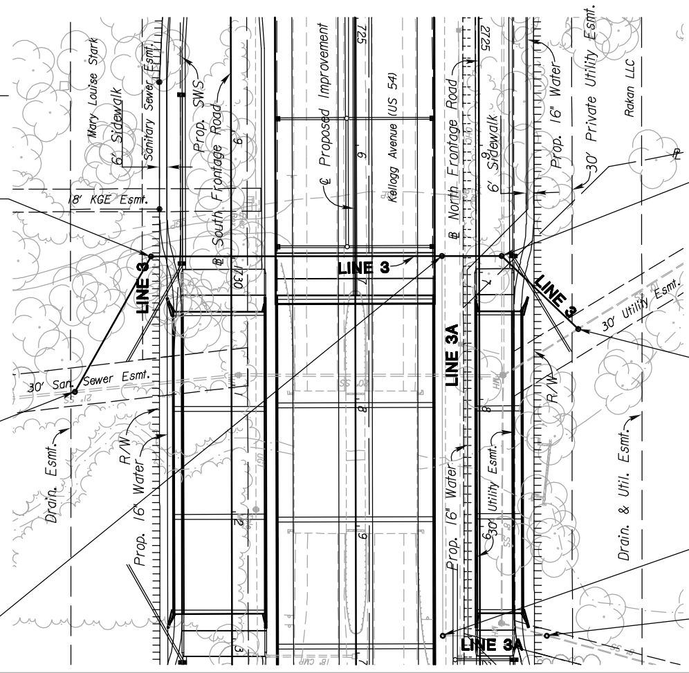
PLAN - LINE 3 SCALE: 1" = 50'
