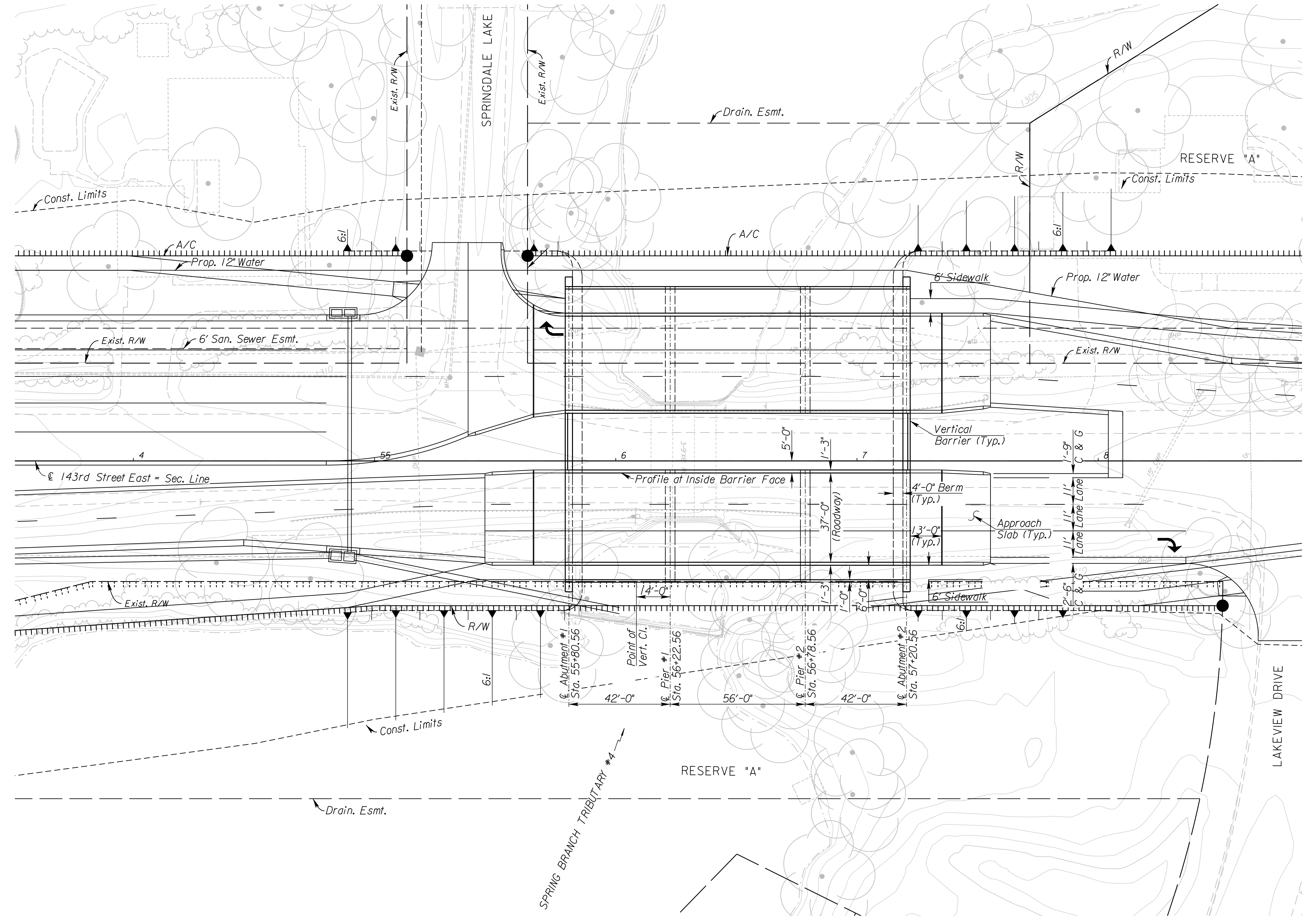
PLAN
