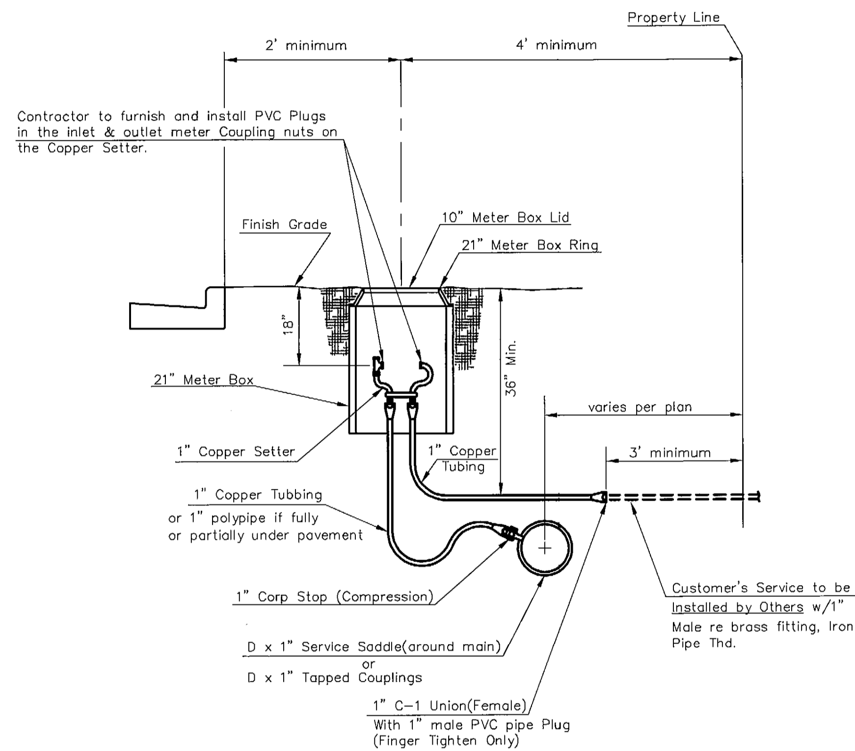
TYPICAL 1" METER SETTING
