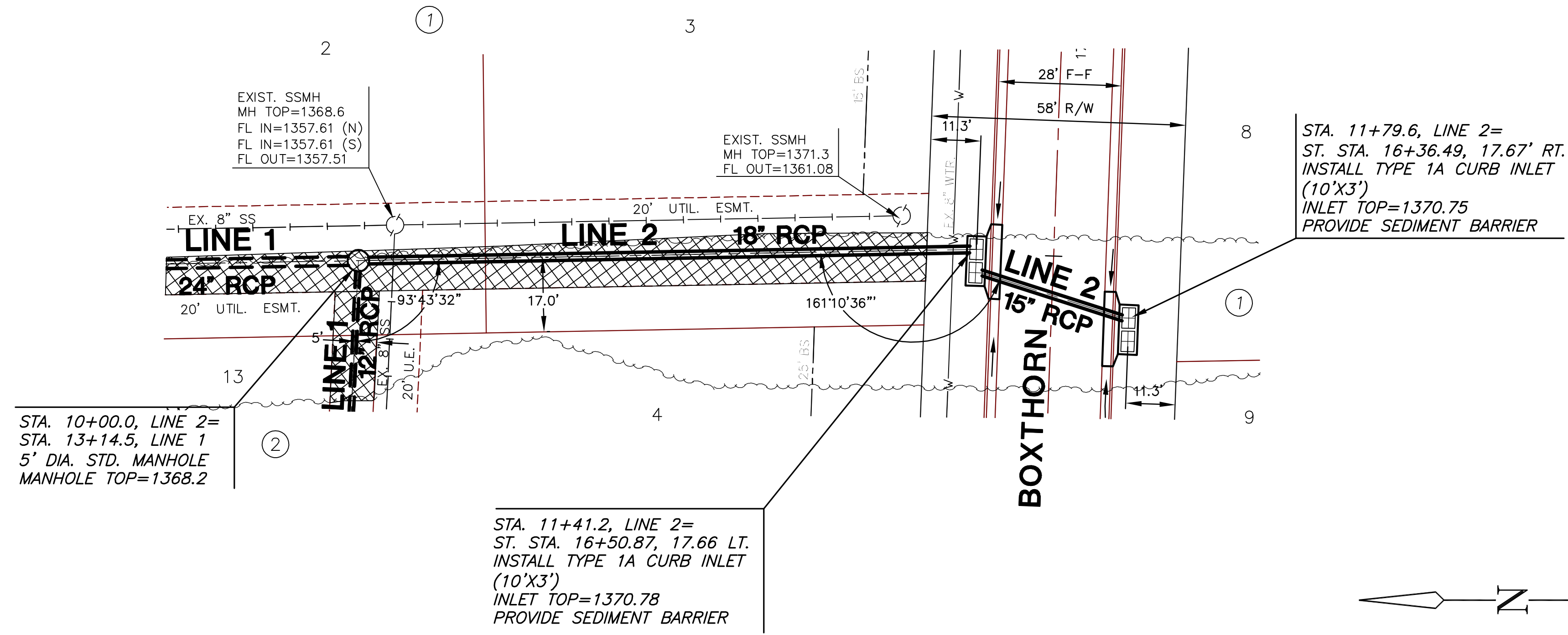
PLAN LINE 2
