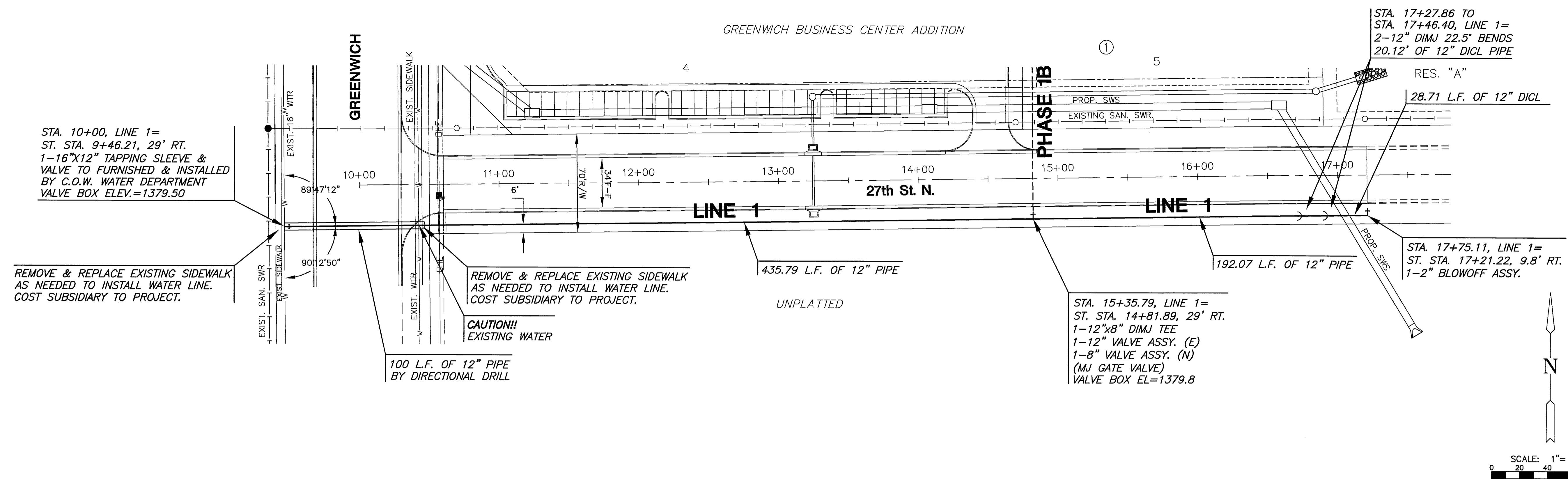
PLAN LINE 1 PROFILE LINE 1
