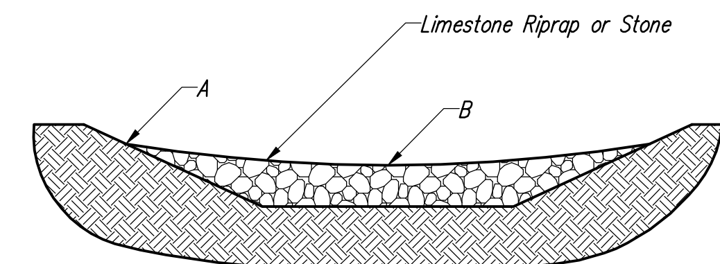
INSTALLATION OF ROCK DITCH CHECKS
