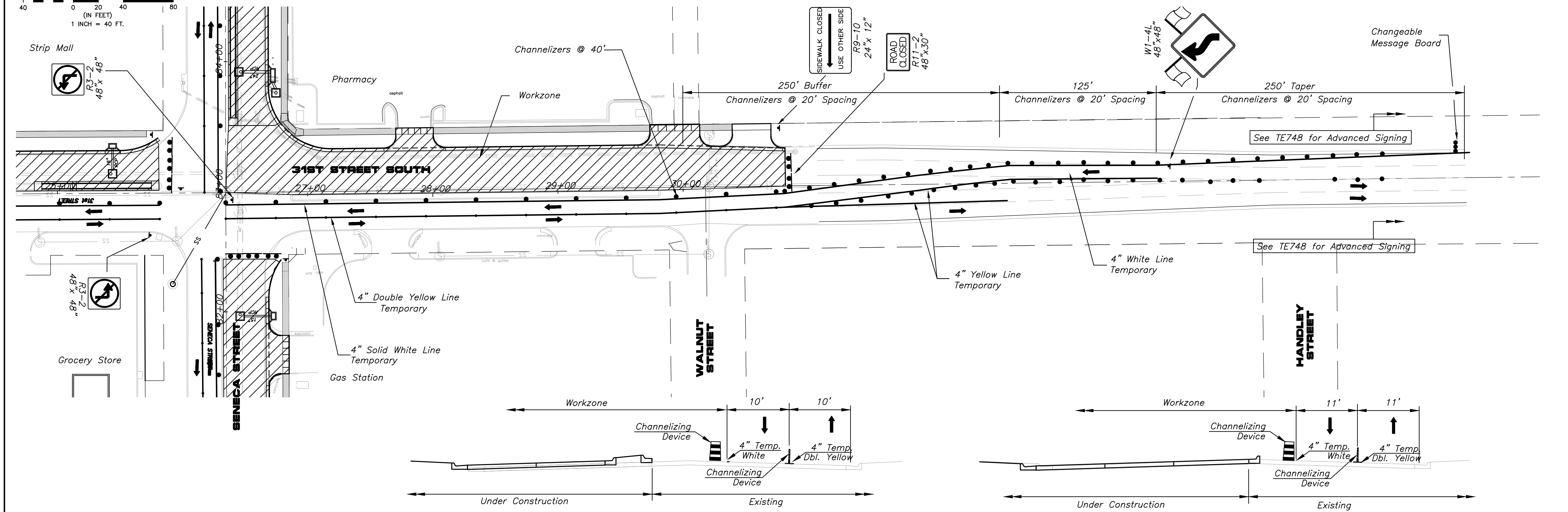
Phase 2 Traffic Control Section Looking East (31st Street South)
