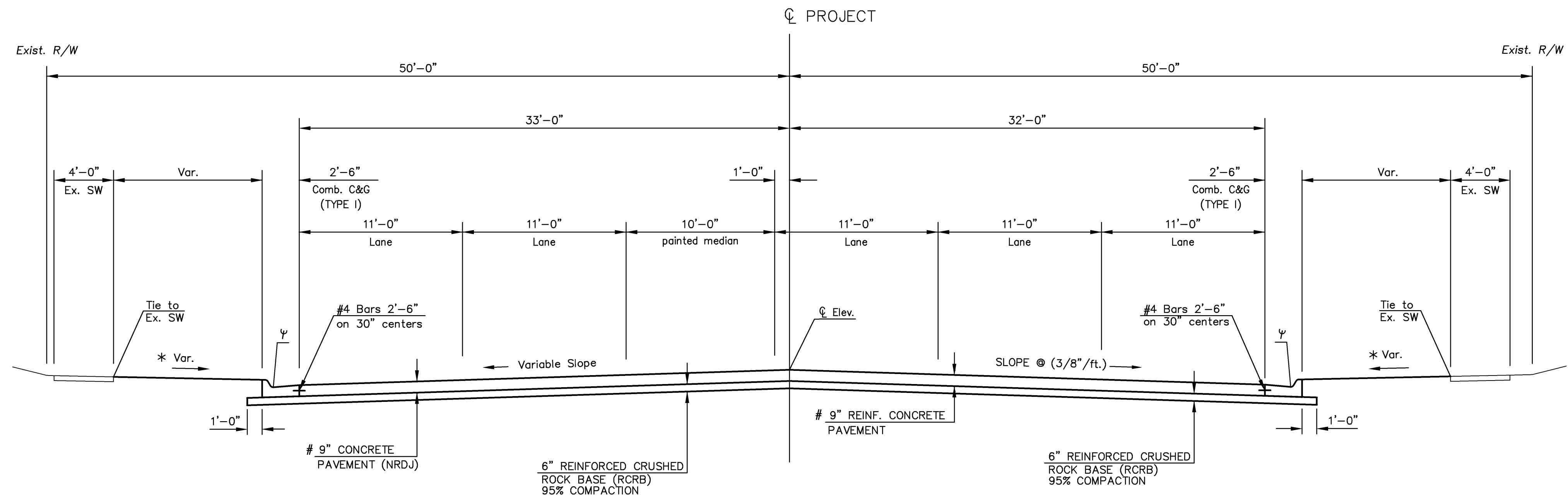
TYPICAL SECTION HARRY ST. Sta. 106+09.65 to Sta. 108+48.82
