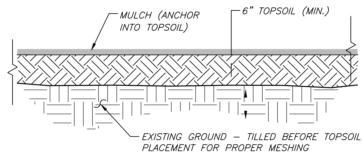
TYPICAL FILL SECTION
