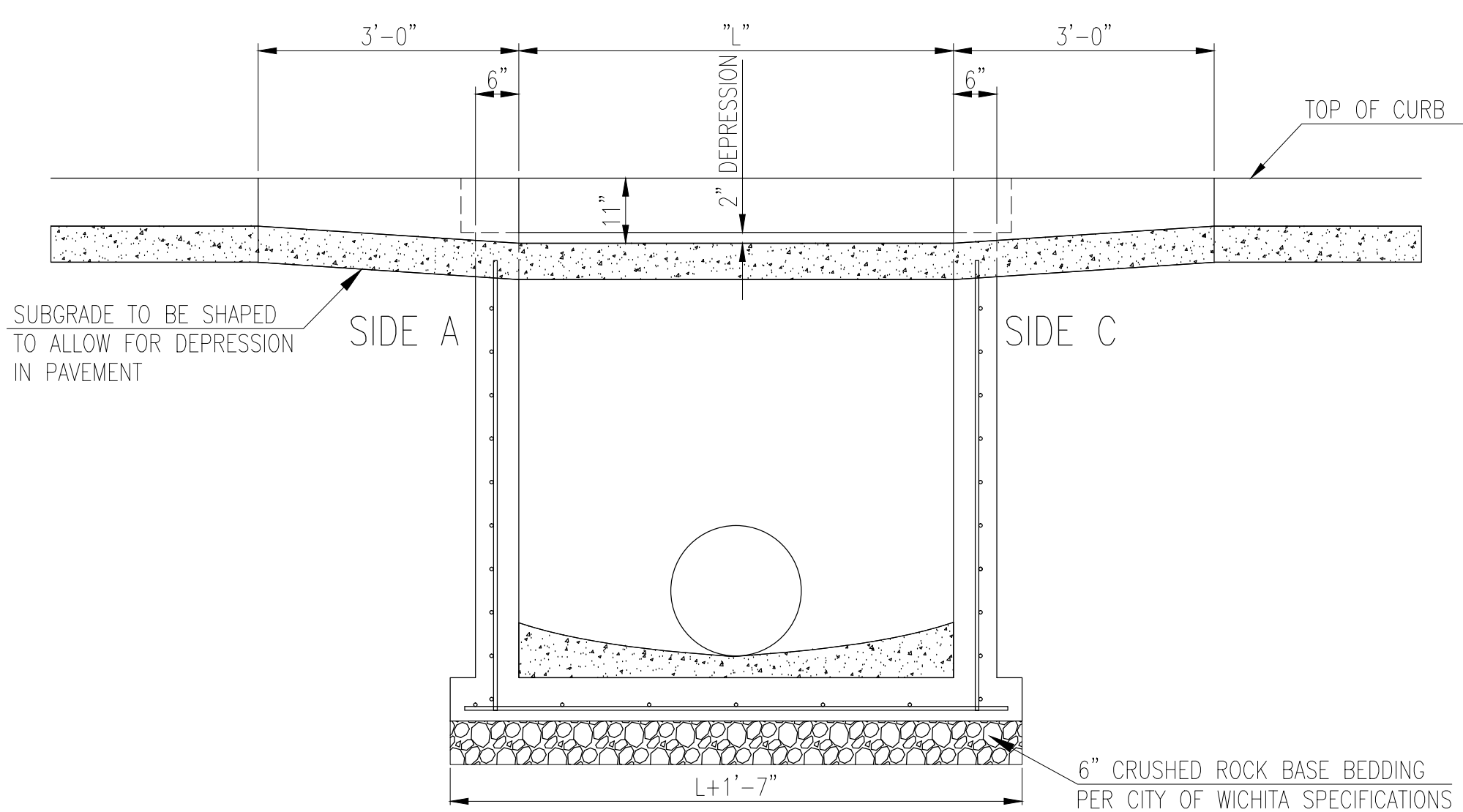
SECTION "B-B"
