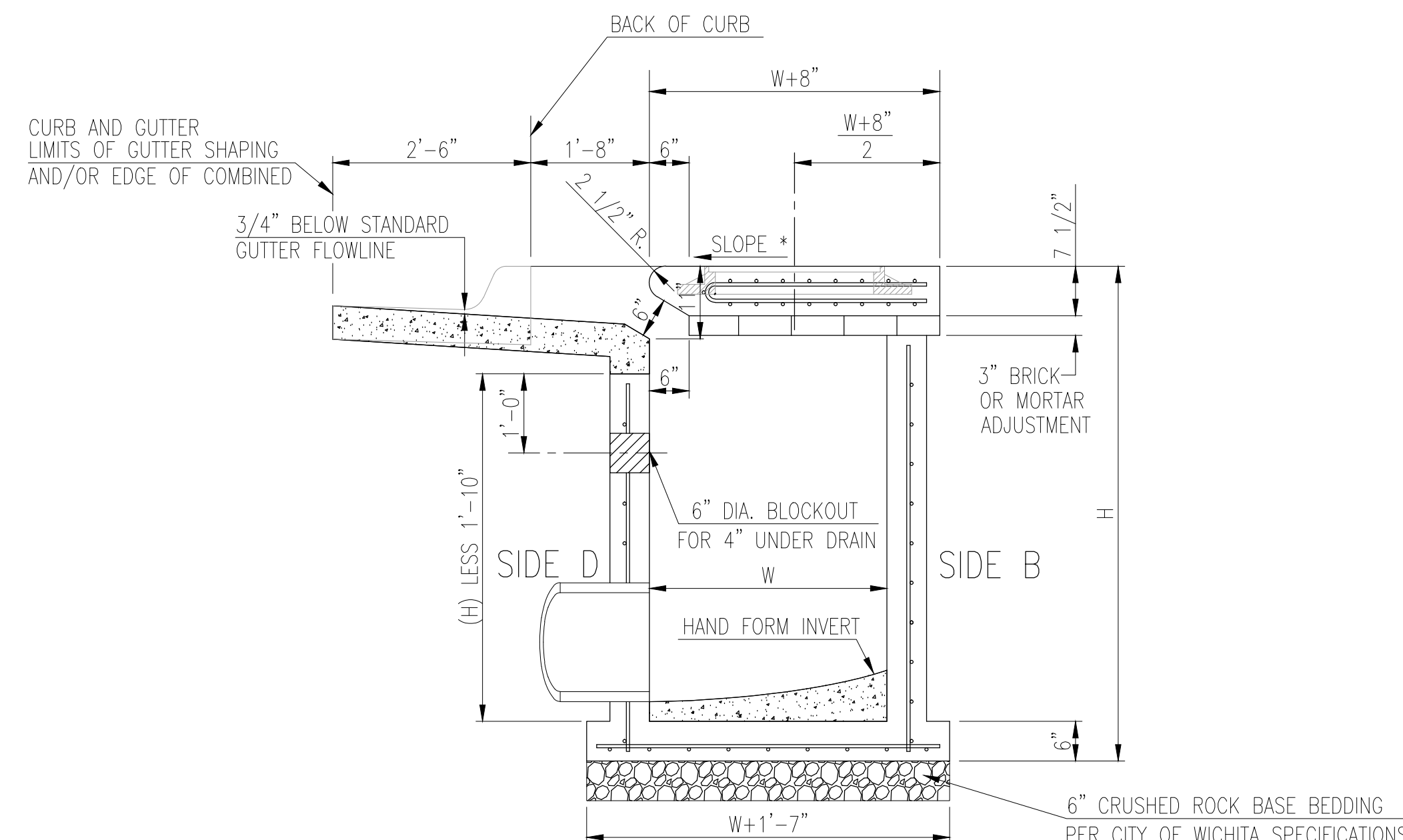
SECTION "C-C"
