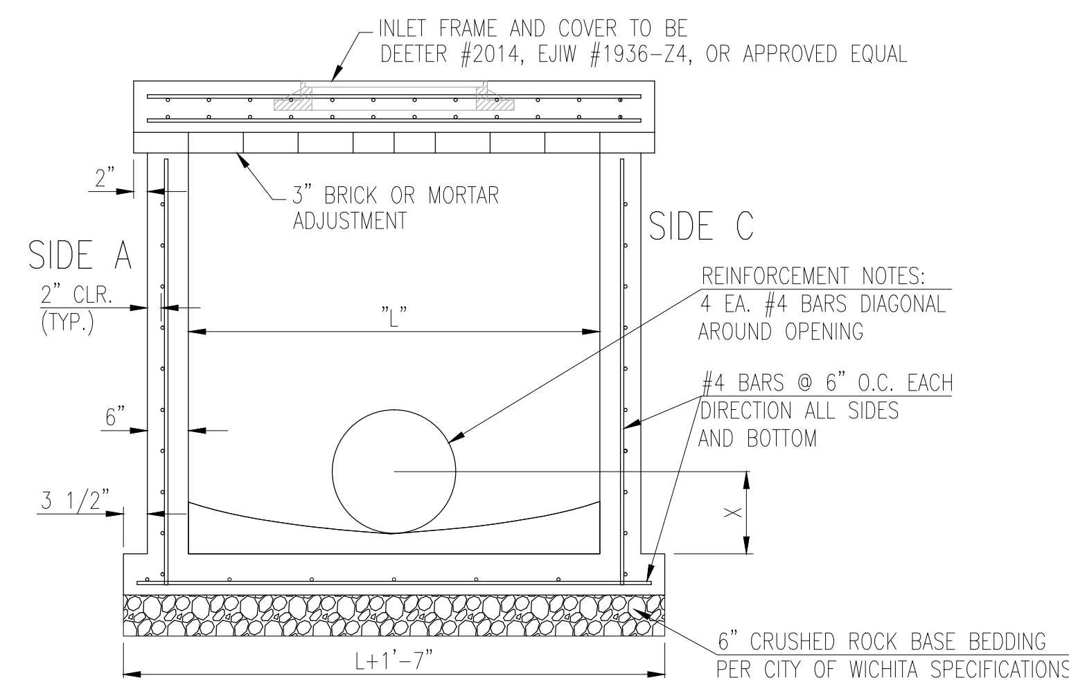
SECTION "A-A"
