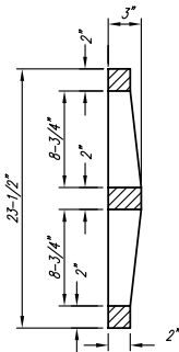
24" x 24" Frame and Grate Detail
