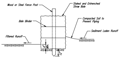
STRAW BALE BARRIERS
