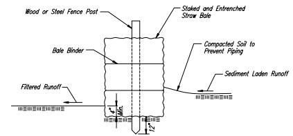
STRAW BALE BARRIERS
