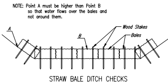
STRAW BALE DITCH CHECKS
