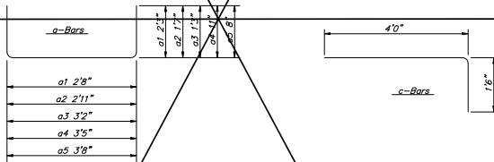
REBAR SCHEDULE
