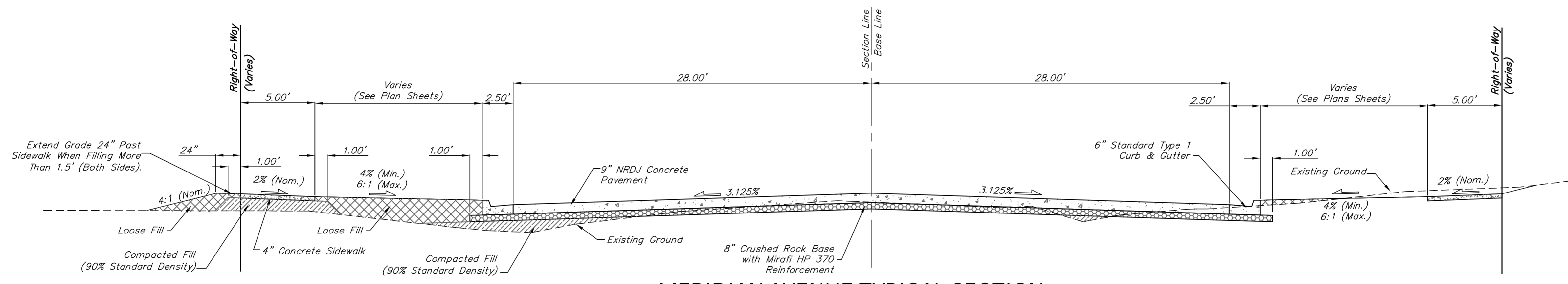
MERIDIAN AVENUE TYPICAL SECTION Sta. 40+85.00 to Sta. 42+88.40
