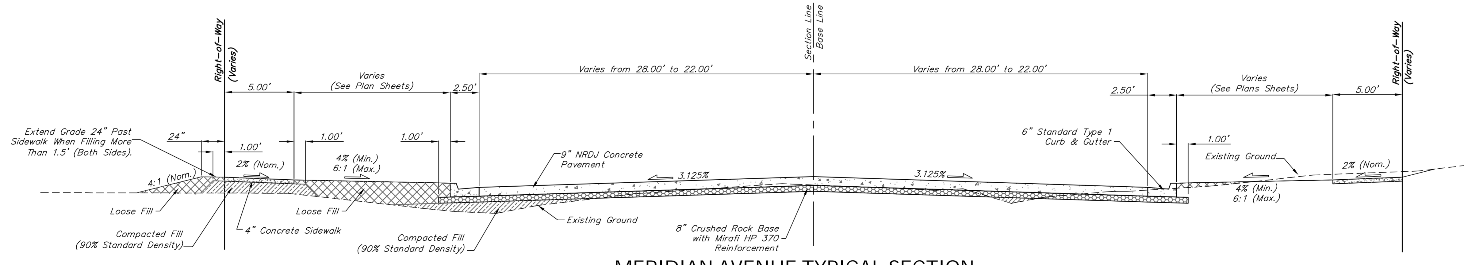
MERIDIAN AVENUE TYPICAL SECTION Sta. 42+88.40 to Sta. 44+07.76
