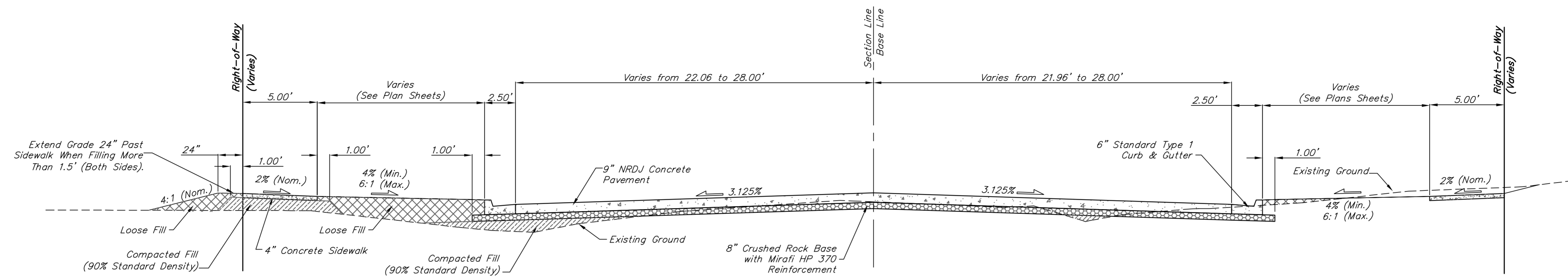
MERIDIAN AVENUE TYPICAL SECTION Sta. 40+55.00 to Sta. 40+85.00
