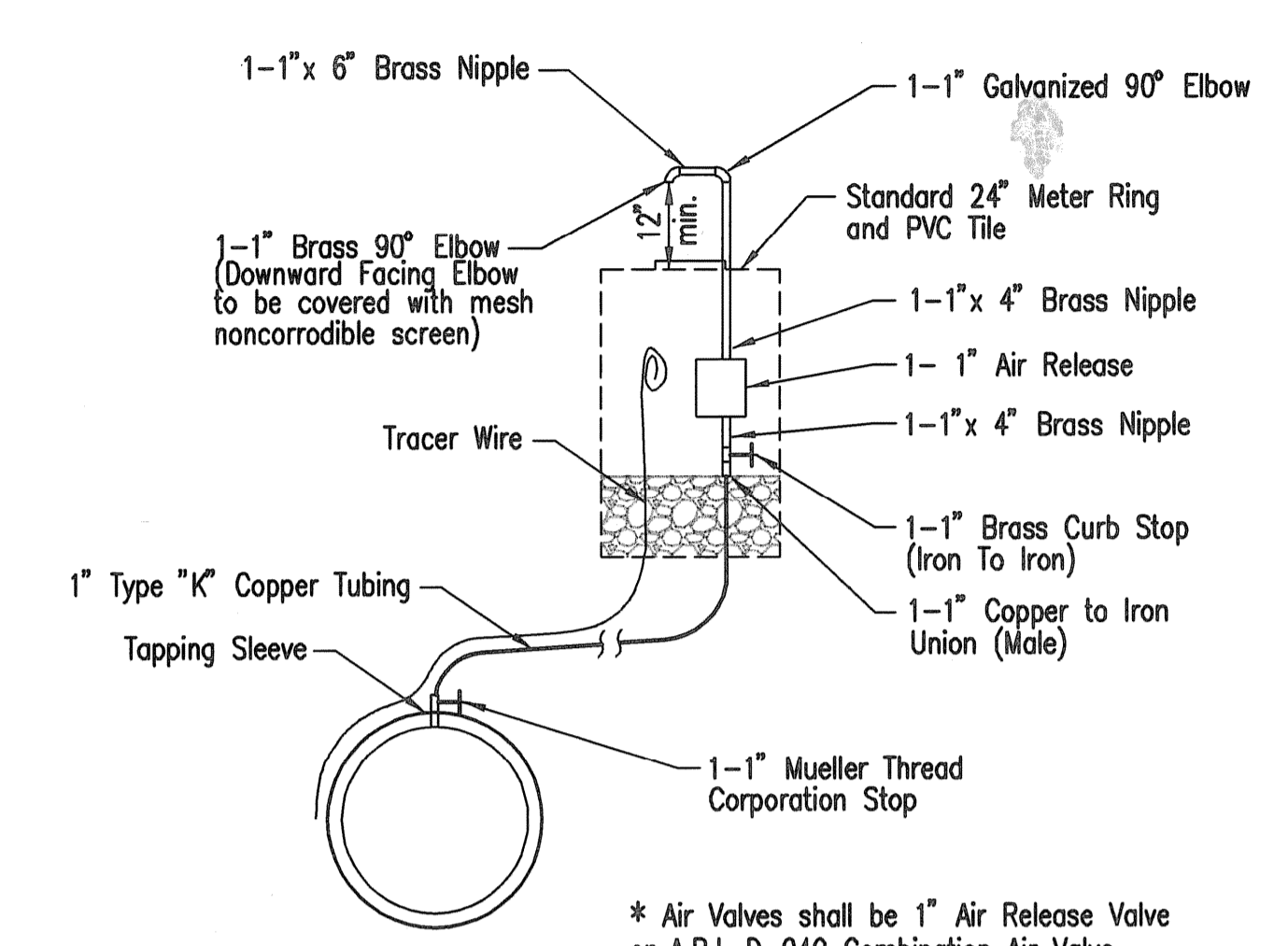
1" AIR RELEASE VALVE ASSEMBLY DETAIL
