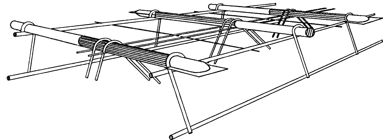
PERSPECTIVE VIEW
