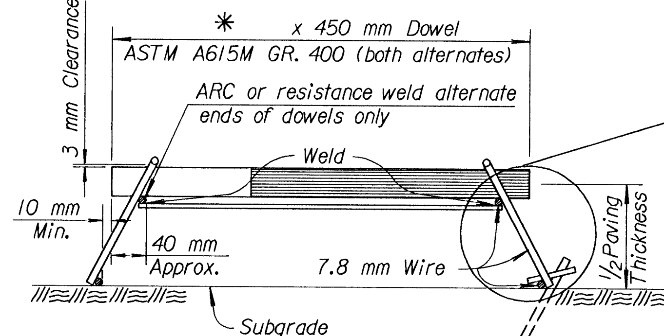
SEC. B-B
