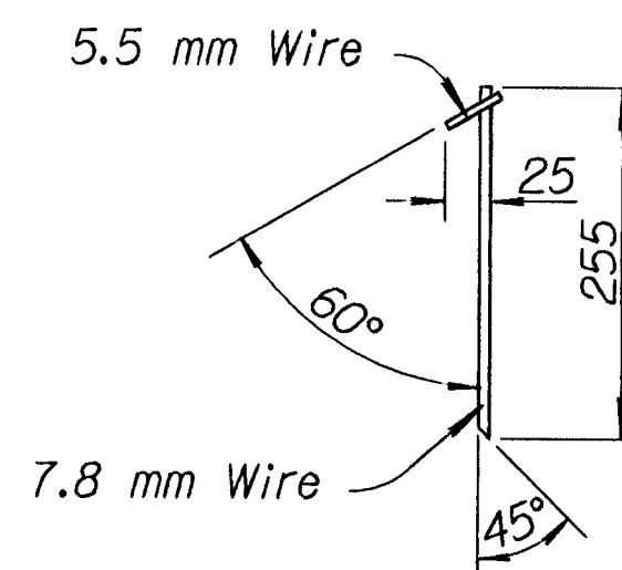
STAKE DETAIL
