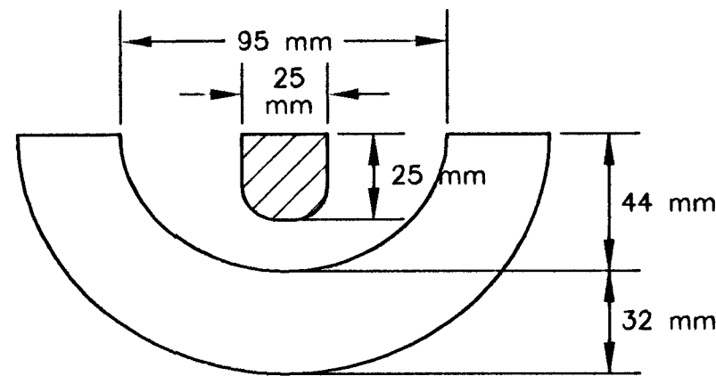
SECTION VIEW
