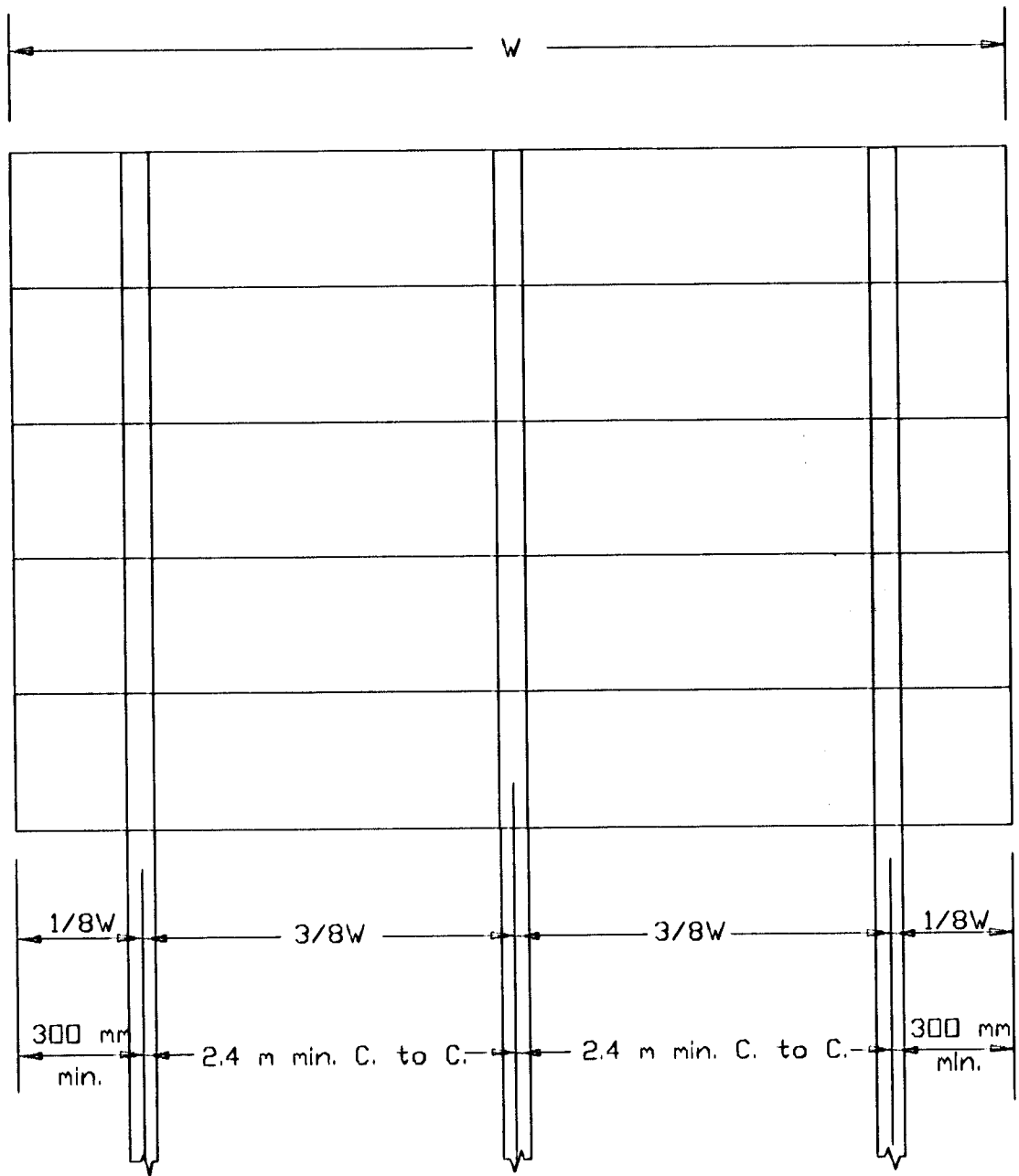
THREE POST SPACING (SEE GENERAL NOTE)
