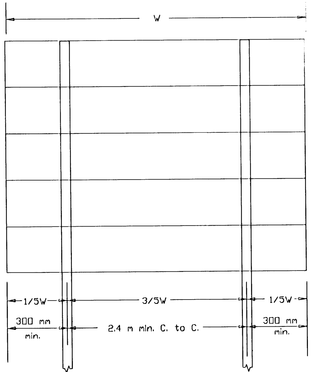
TWO POST SPACING (SEE GENERAL NOTE)
