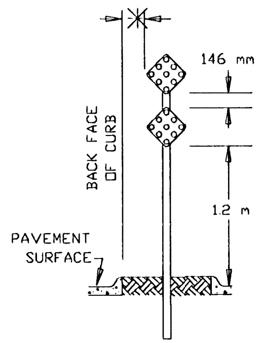
MEDIAN INSTALLED TWO T1/DM
