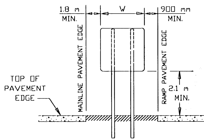
GORE INSTALLED SIGN (BETWEEN MAINLINE AND RAMP)
