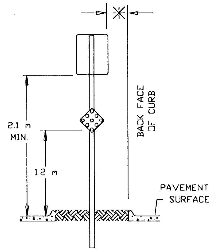
MEDIAN INSTALLED SIGN WITH ONE T1/DM
