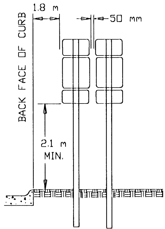
SHOULDER INSTALLED ROUTE MARKER DIRECTIONAL SIGNS
