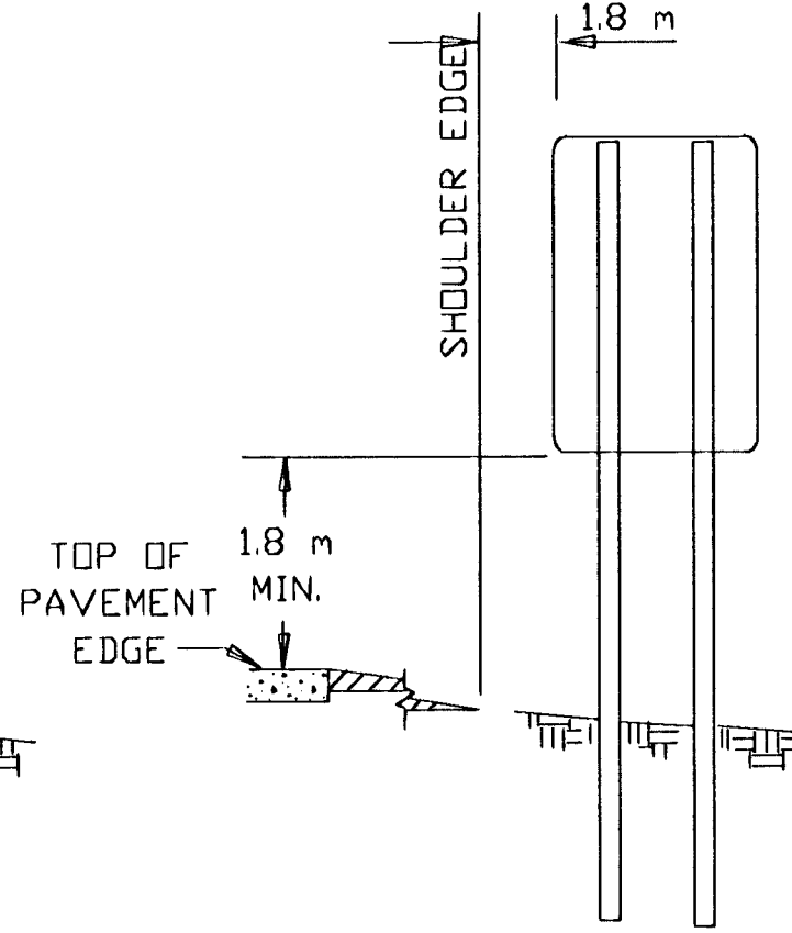
SHOULDER INSTALLED SPEED LIMIT SIGN
