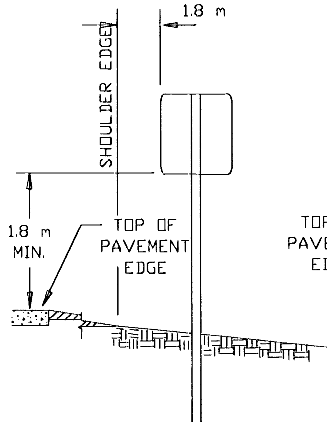
SHOULDER INSTALLED SIGN
