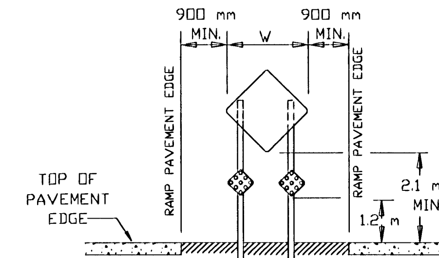
GORE INSTALLED SIGN WITH TWO T1/DM'S (BETWEEN TWO RAMP)
