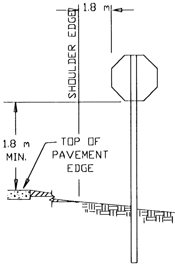
SHOULDER INSTALLED STOP SIGN
