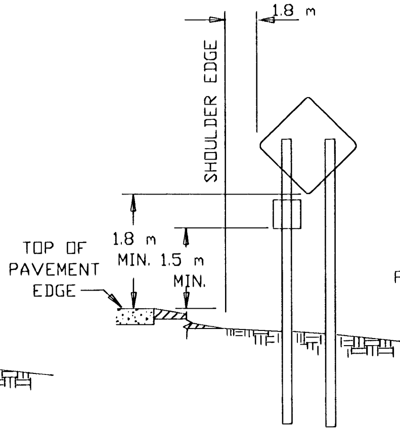
SHOULDER INSTALLED DIAMOND SIGN WITH OR WITHOUT AUX. SIGN
