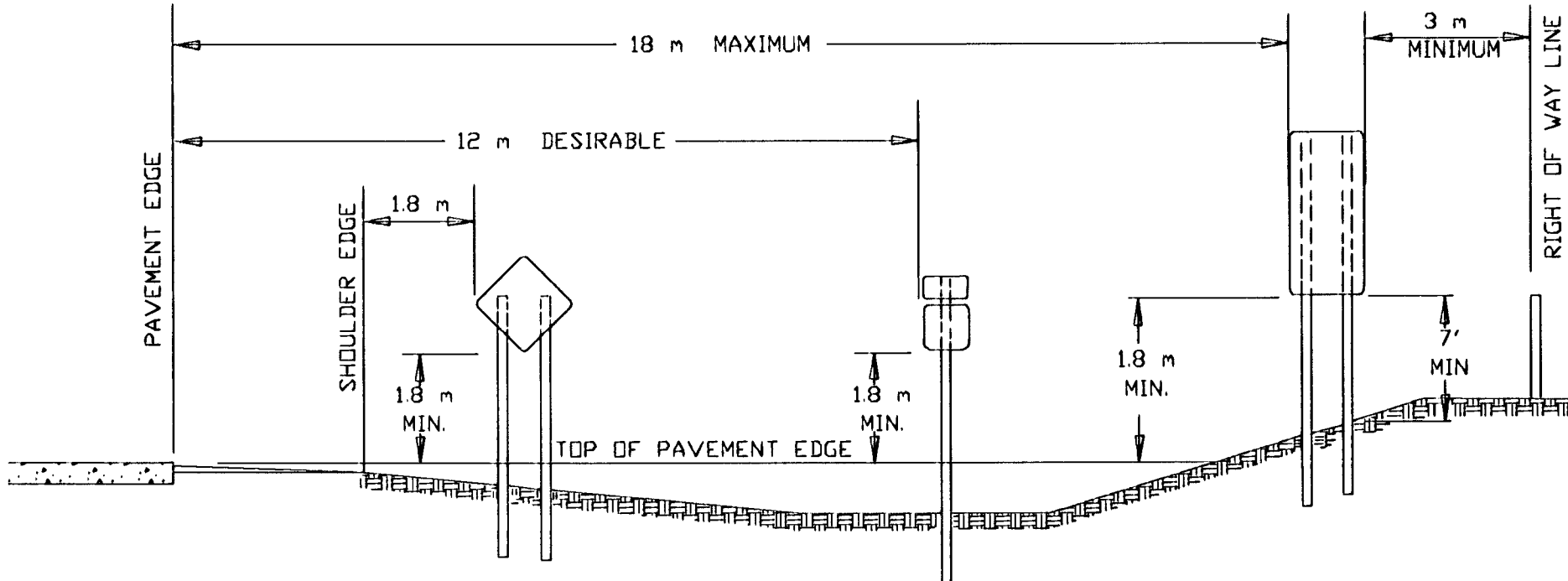
MAINLINE INSTALLED REGULATORY SIGNS, WARNING SIGNS OR ROUTE MARKERS
