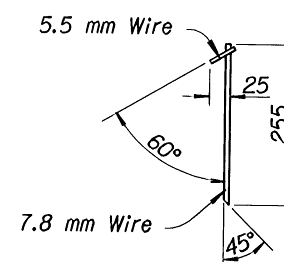
STAKE DETAIL
