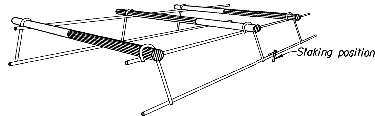
PERSPECTIVE VIEW
