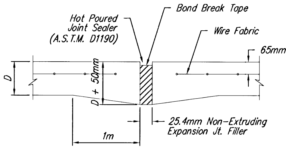
EXPANSION JOINT
