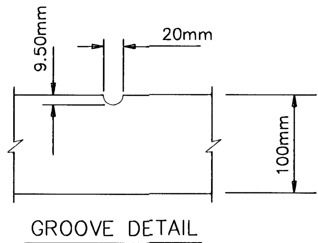
GROOVE DETAIL
