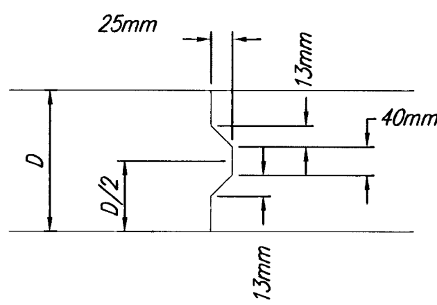
KEYWAY DETAIL
