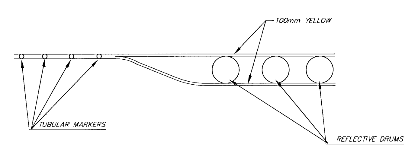
TRANSITION DETAILS TUBULAR MARKERS TO REFLECTIVE DRUMS (NTS)
