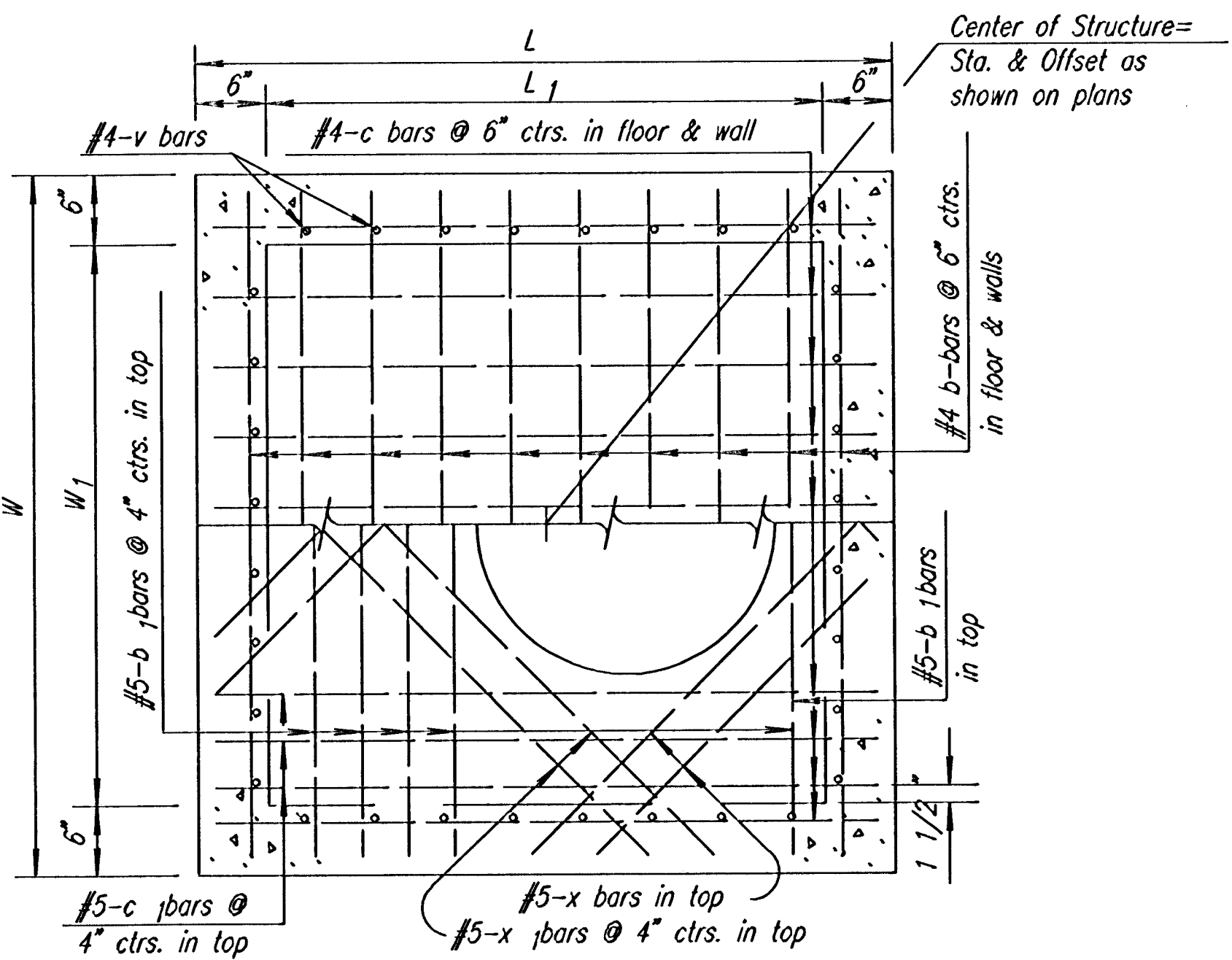
PLAN (Showing top & floor reinf.)
