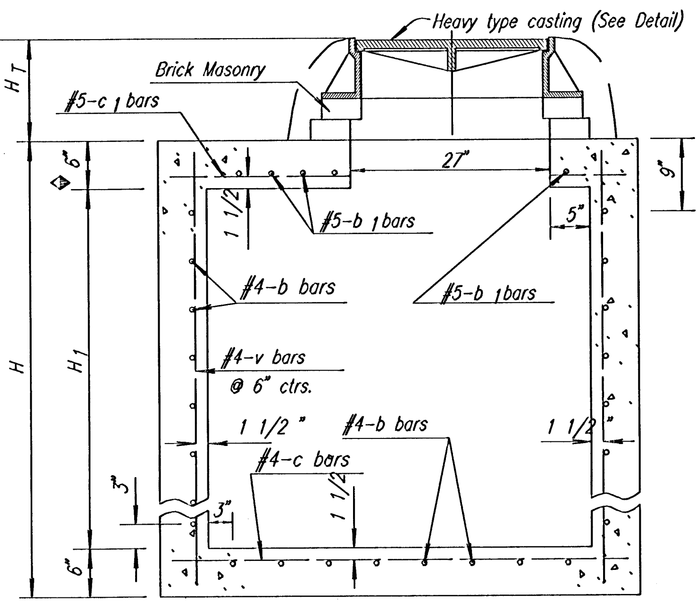
SECTION (Exclusive of floor shaping)
