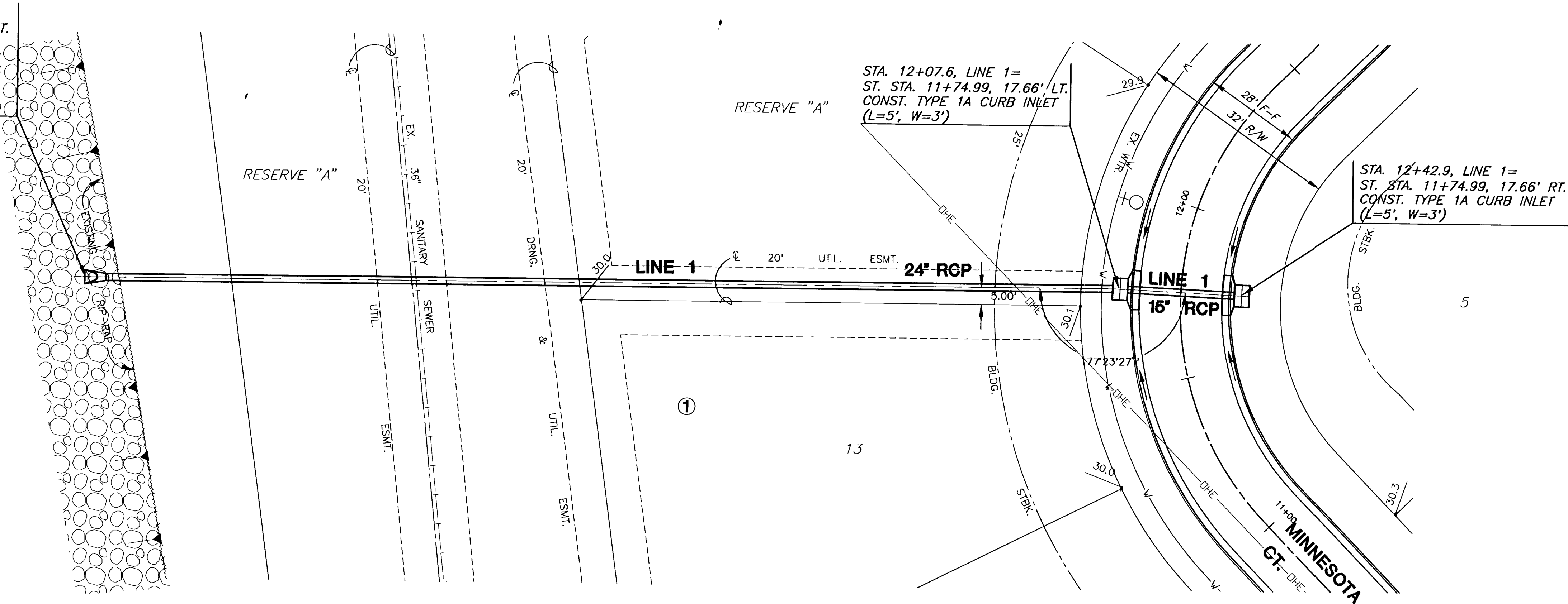
PLAN - LINE 1 SCALE: 1" = 20'
