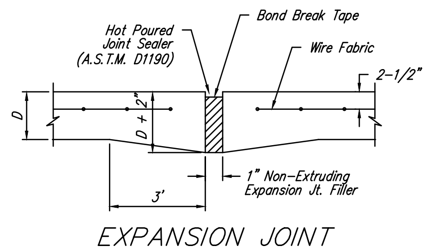
EXPANSION JOINT
