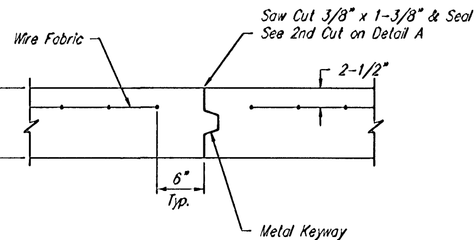
OPTIONAL CONTRACTION JOINT (CONSTRUCTION JOINT)
