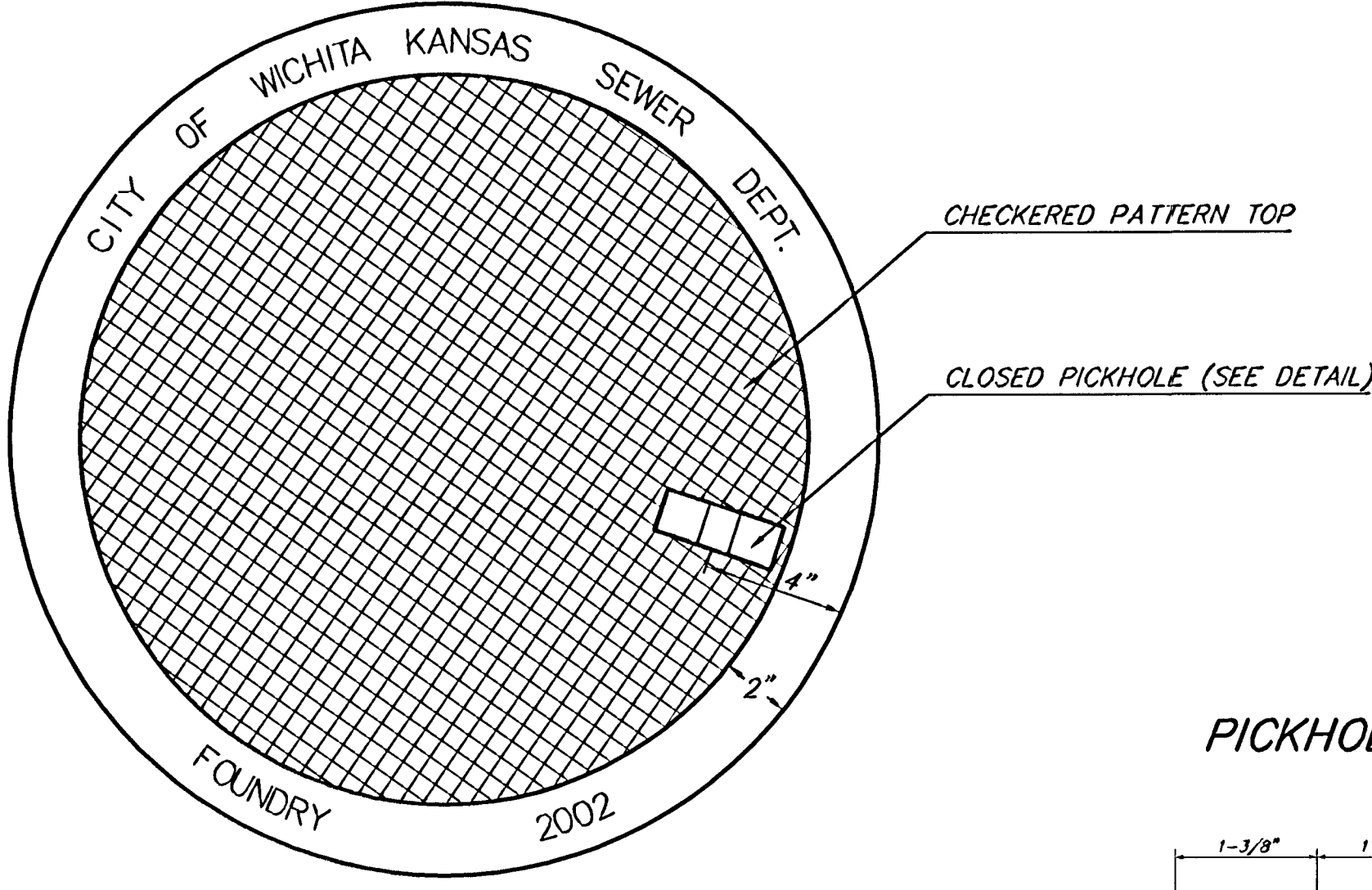
TOP VIEW
