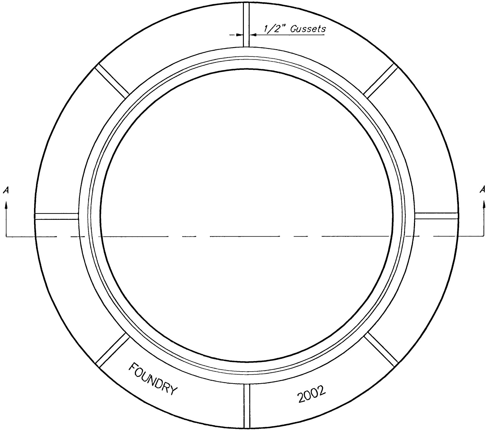
TOP VIEW
