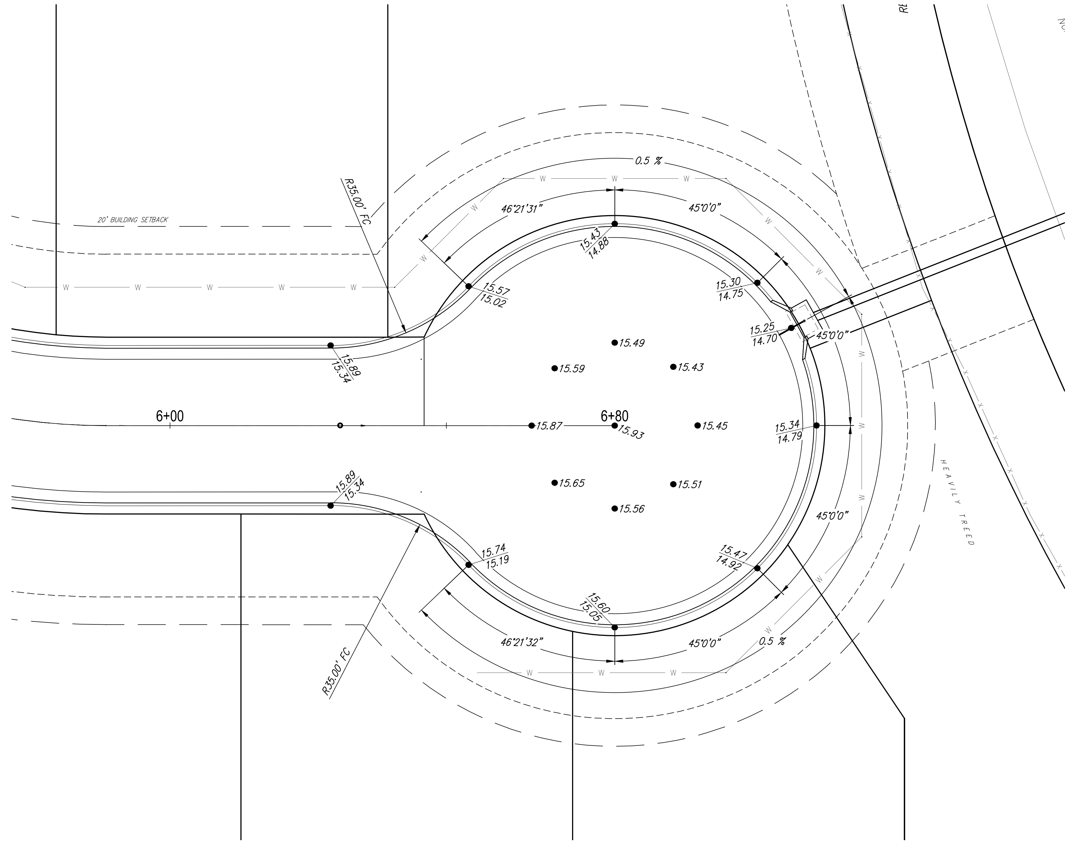
CUL-DE-SAC DETAIL
