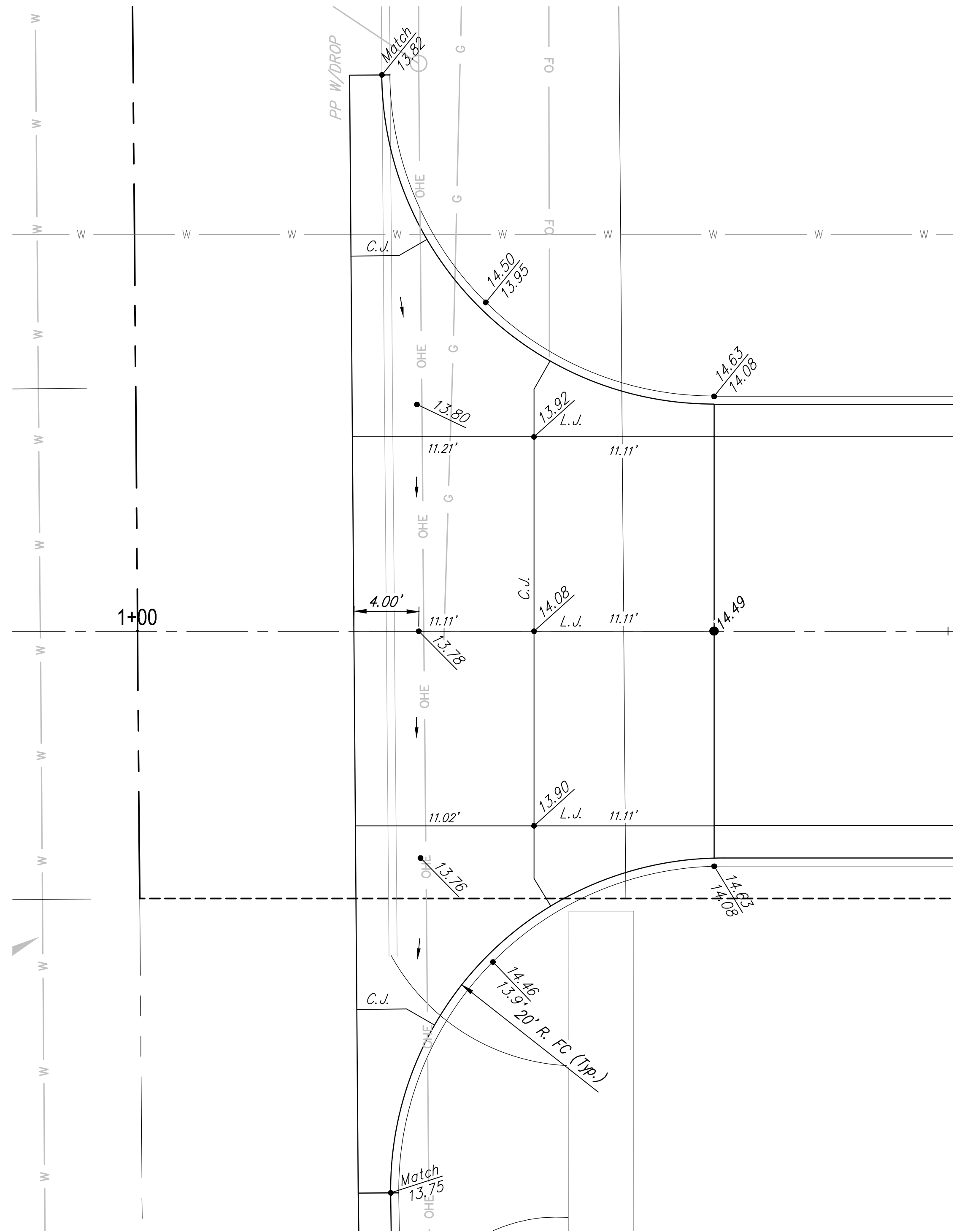
VALLEY GUTTER DETAIL
