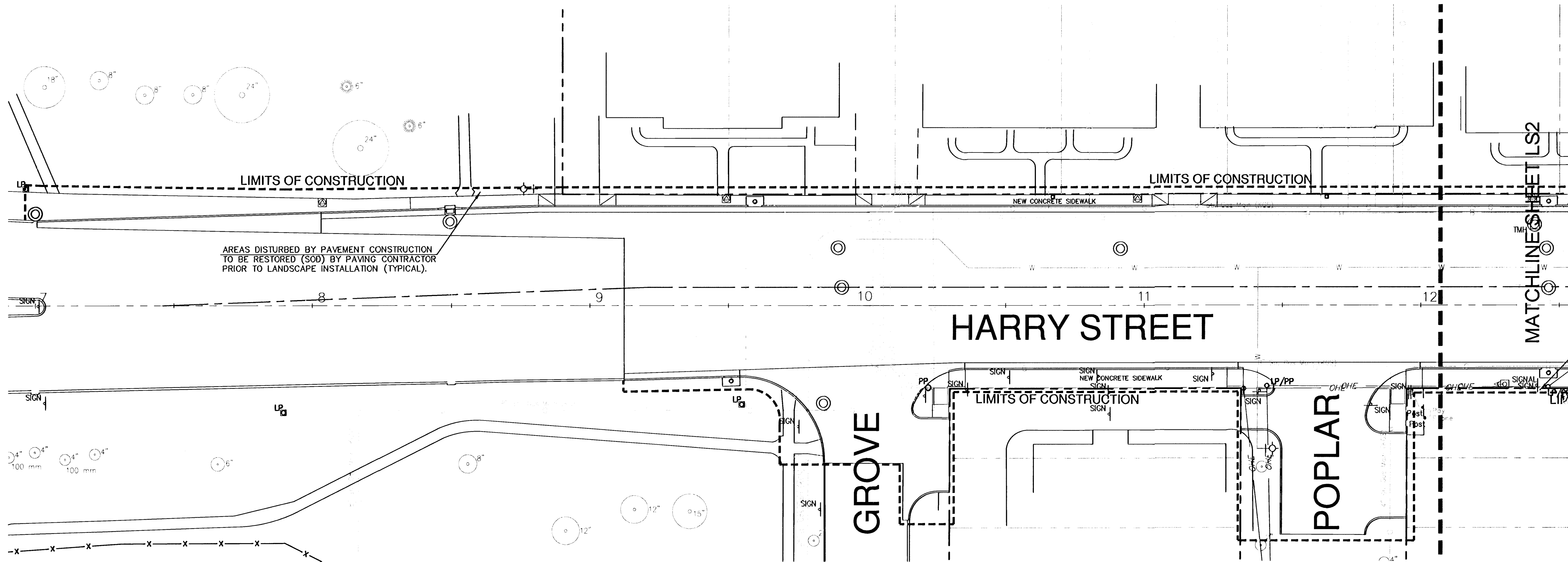
STREET PLANTING PLAN SCALE: 1"=20'-0"
