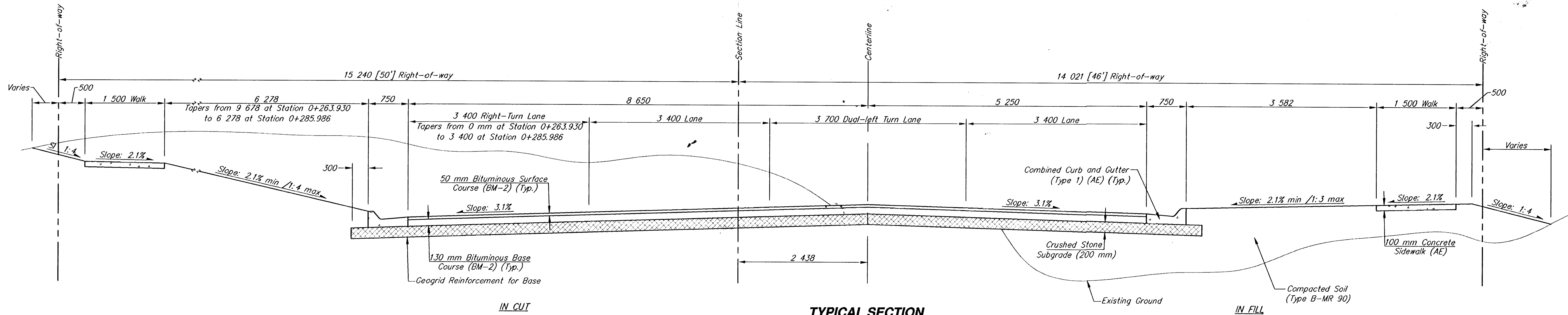
TYPICAL SECTION MERIDIAN - STATION 0+263.930 TO 0+401.137
