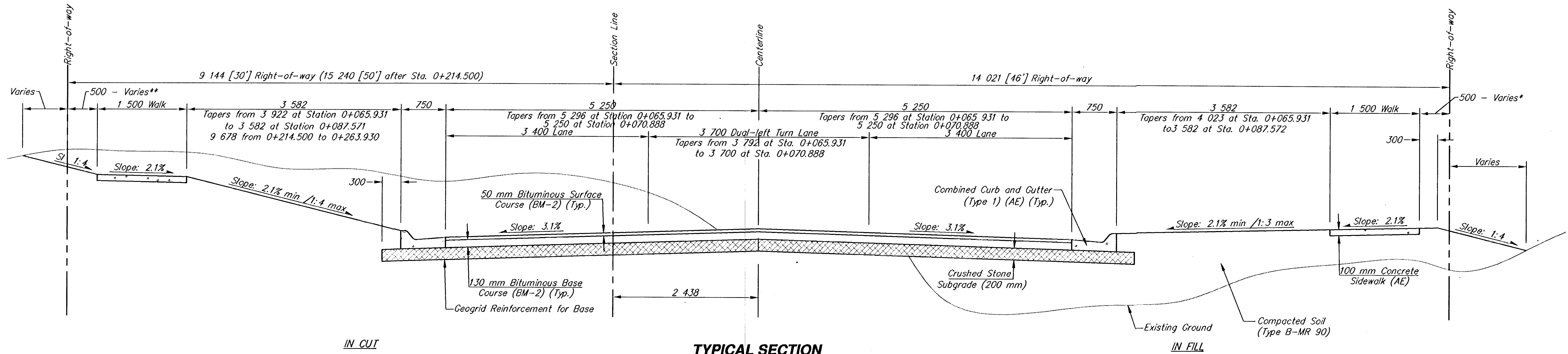
TYPICAL SECTION MERIDIAN - STATION 0+065.931 TO 0+263.930 MERIDIAN - STATION 0+401.137 TO 0+787.486
