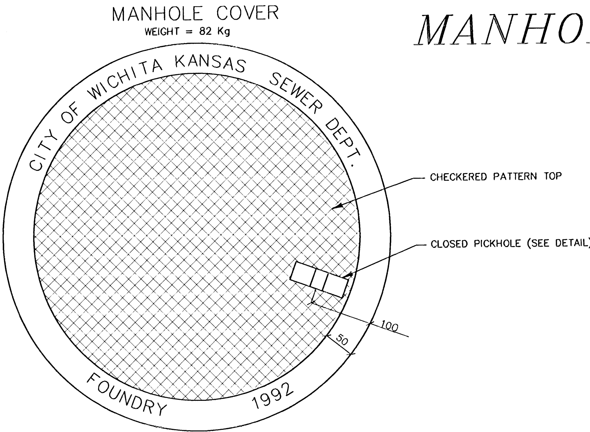
TOP VIEW
