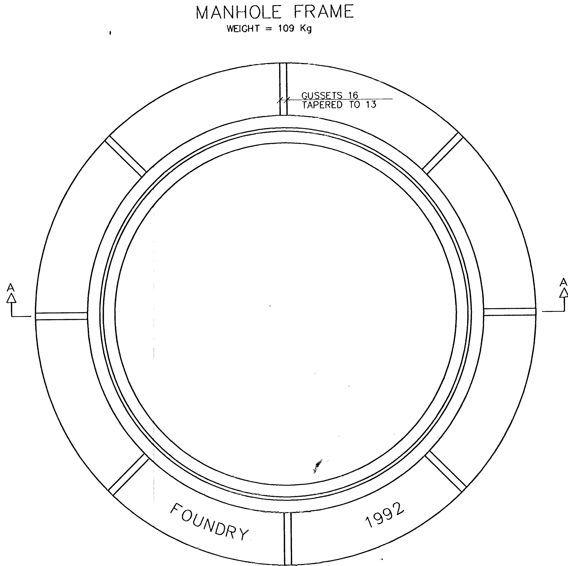
TOP VIEW
