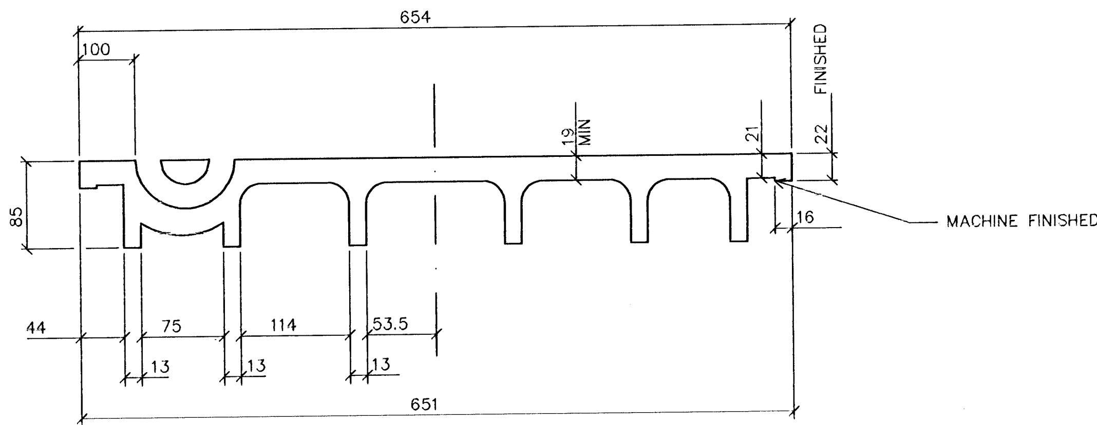
BOTTOM VIEW
