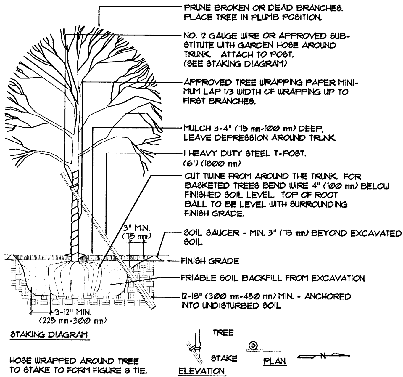
DECIDUOUS TREE PLANTING SMALLER THAN 2" (50 mm) CALIPER
