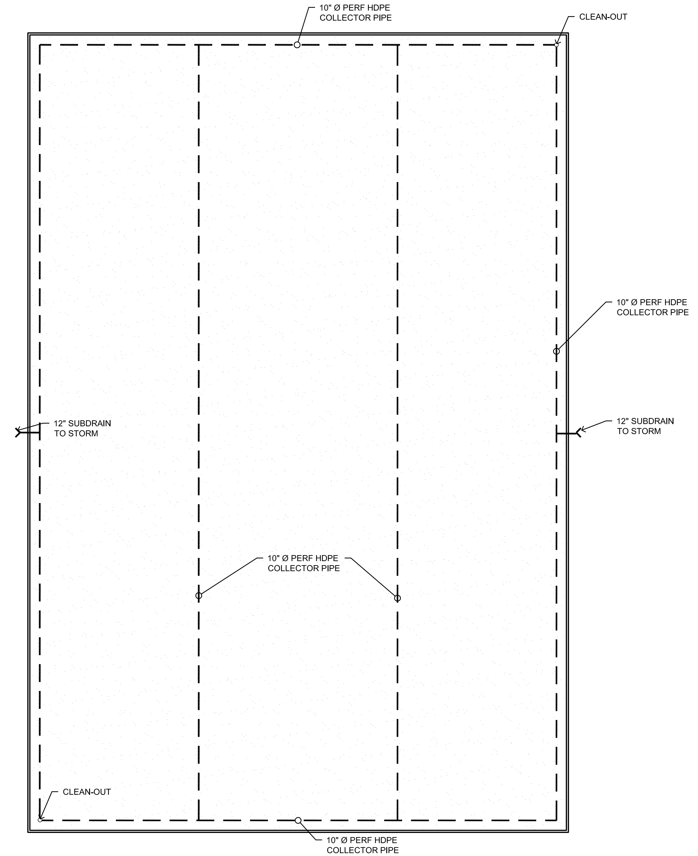
DRAINAGE PLAN
