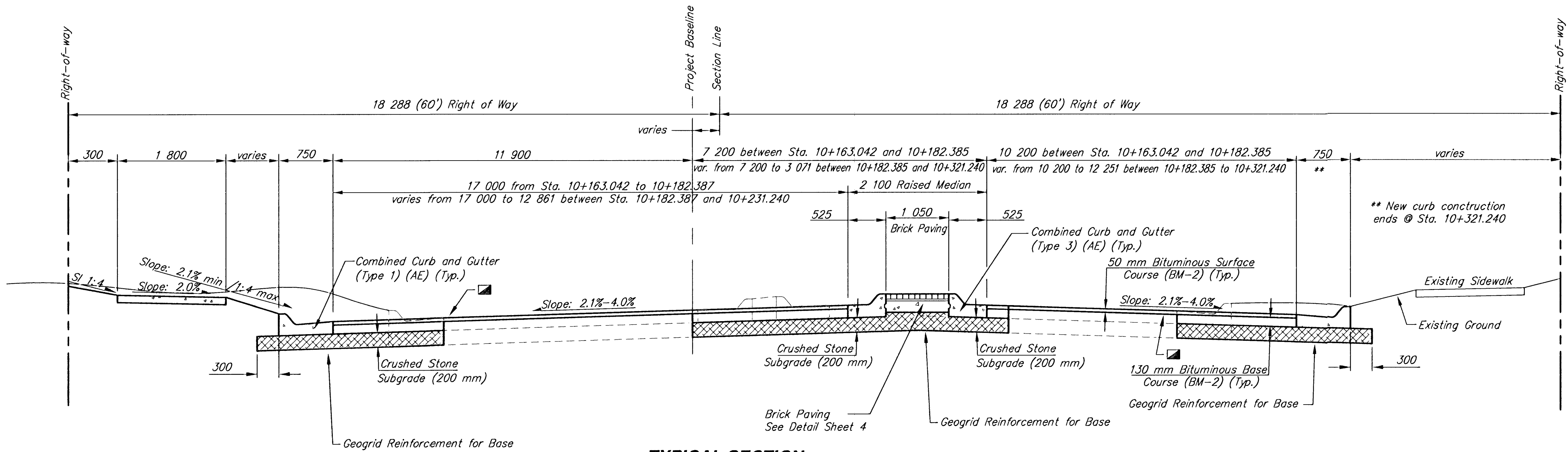
TYPICAL SECTION 10+163.042 TO 10+231.240
