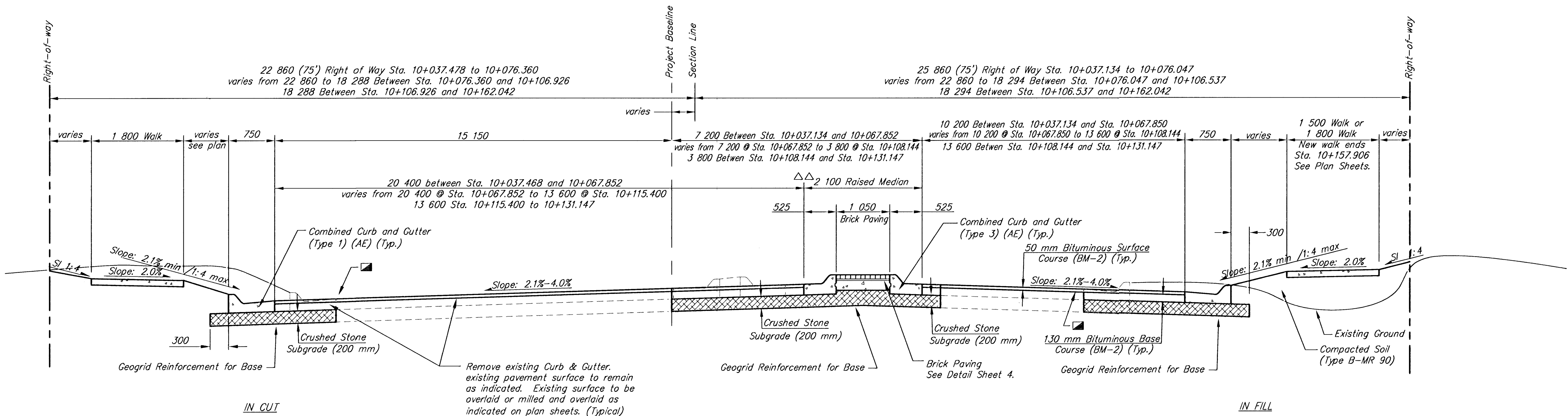
TYPICAL SECTION 10+037.134 TO 10+162.042
