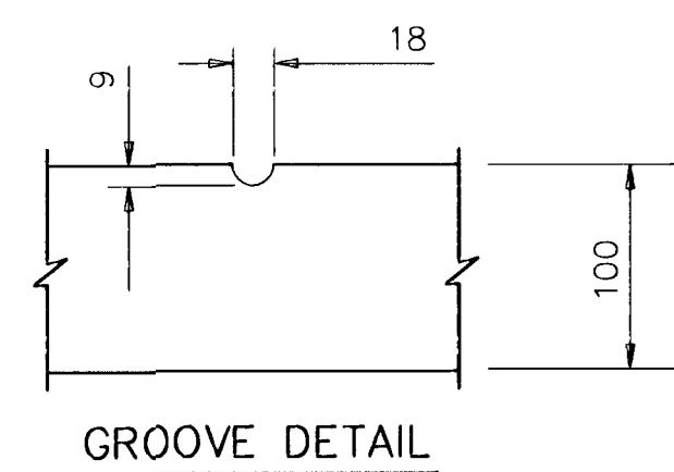
GROOVE DETAIL
