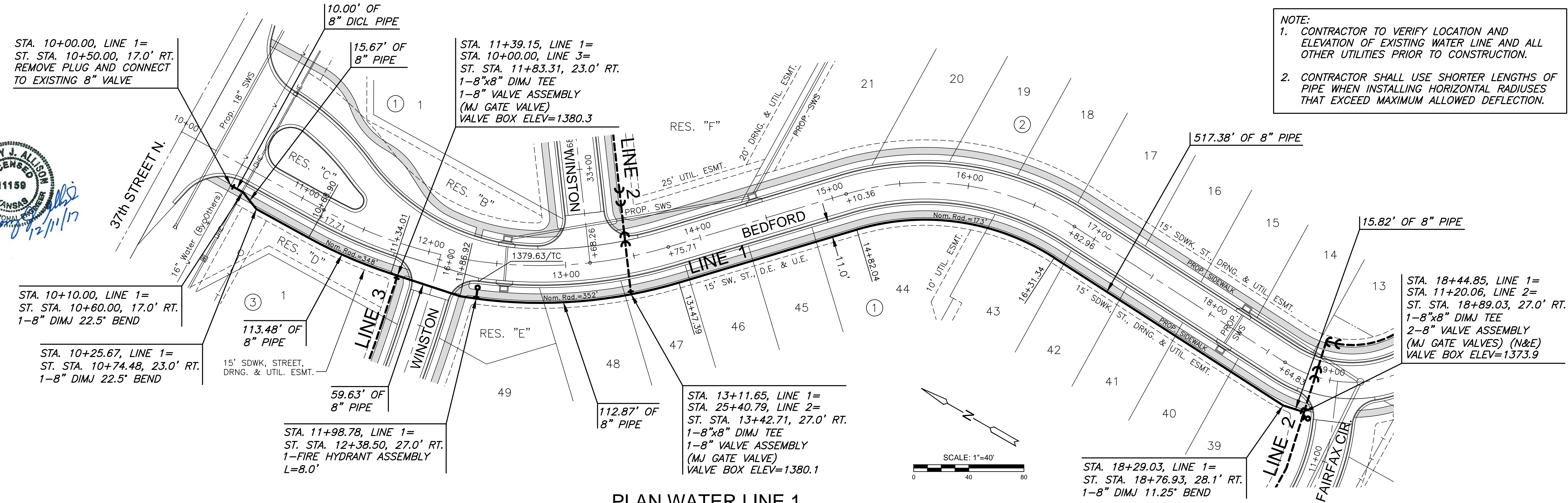
PLAN WATER LINE 1 PROFILE WATER LINE 1
