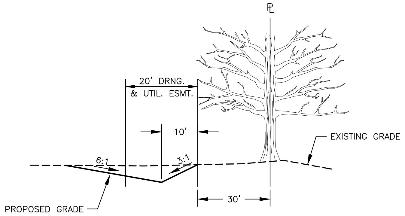
B SOUTH SECTION SCALE: NTS BLOCK 1, LOTS 14 - 30
