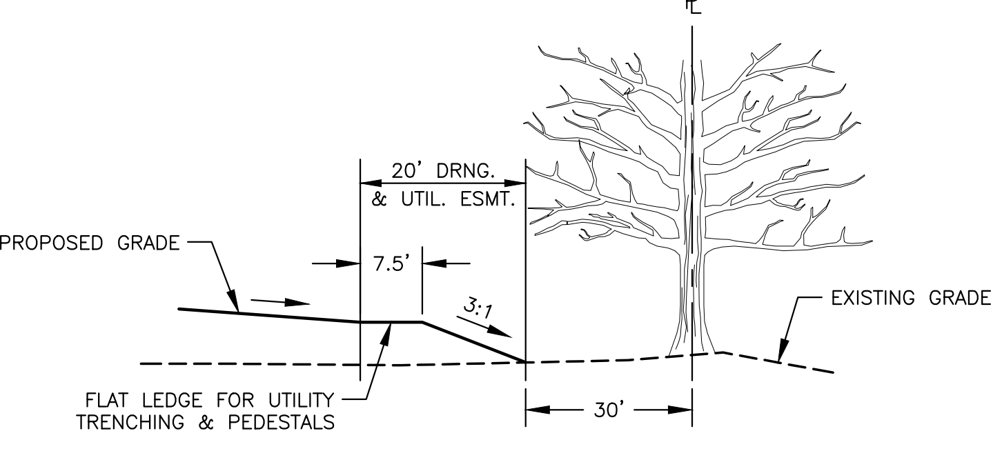
A NORTH SECTION SCALE: NTS BLOCK 1, LOTS 10 - 13
