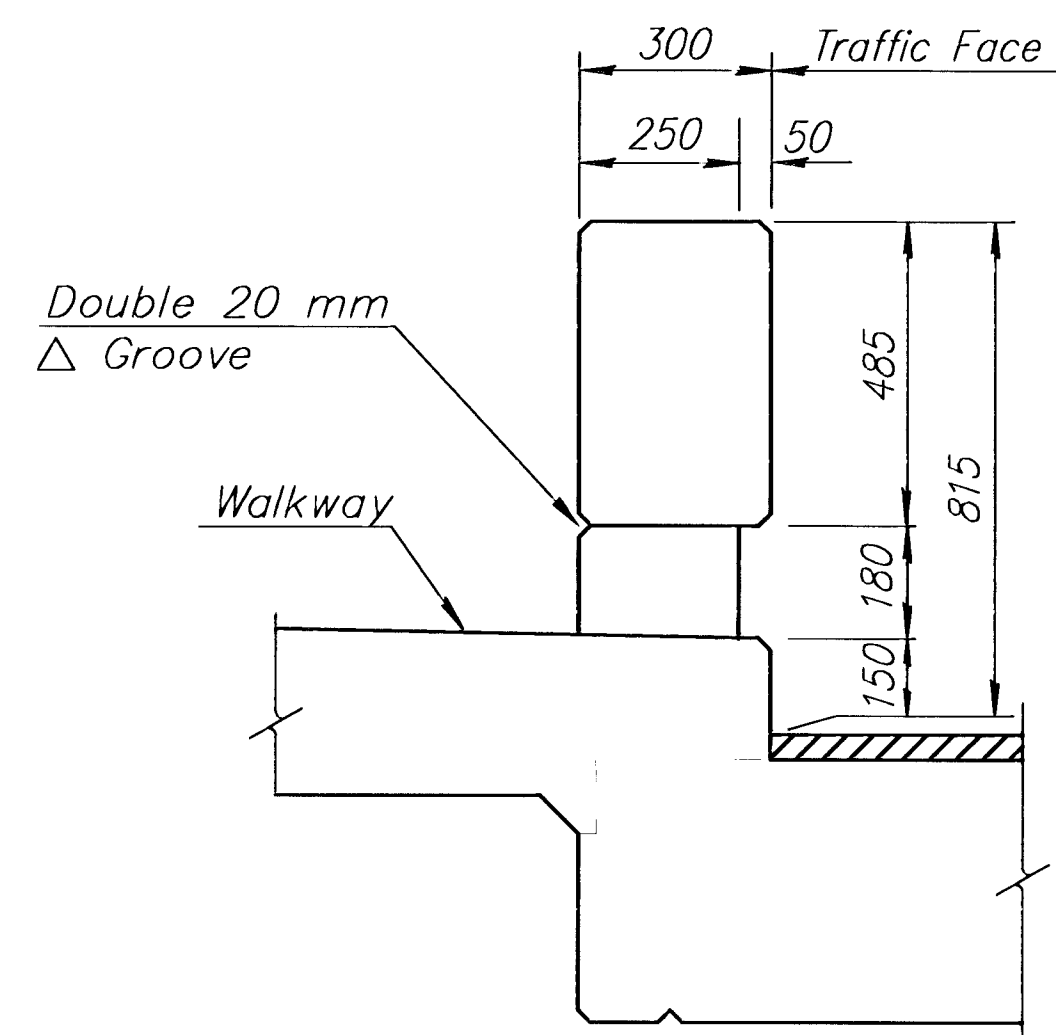
TYPICAL INTERIOR POST
