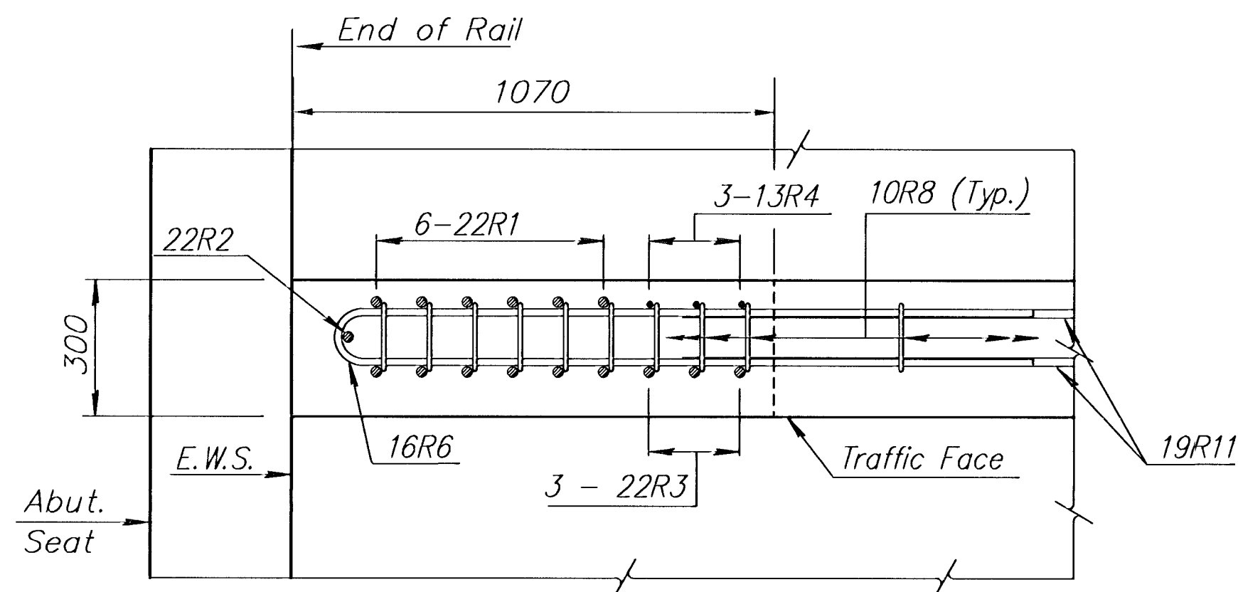
SECTION C-C
