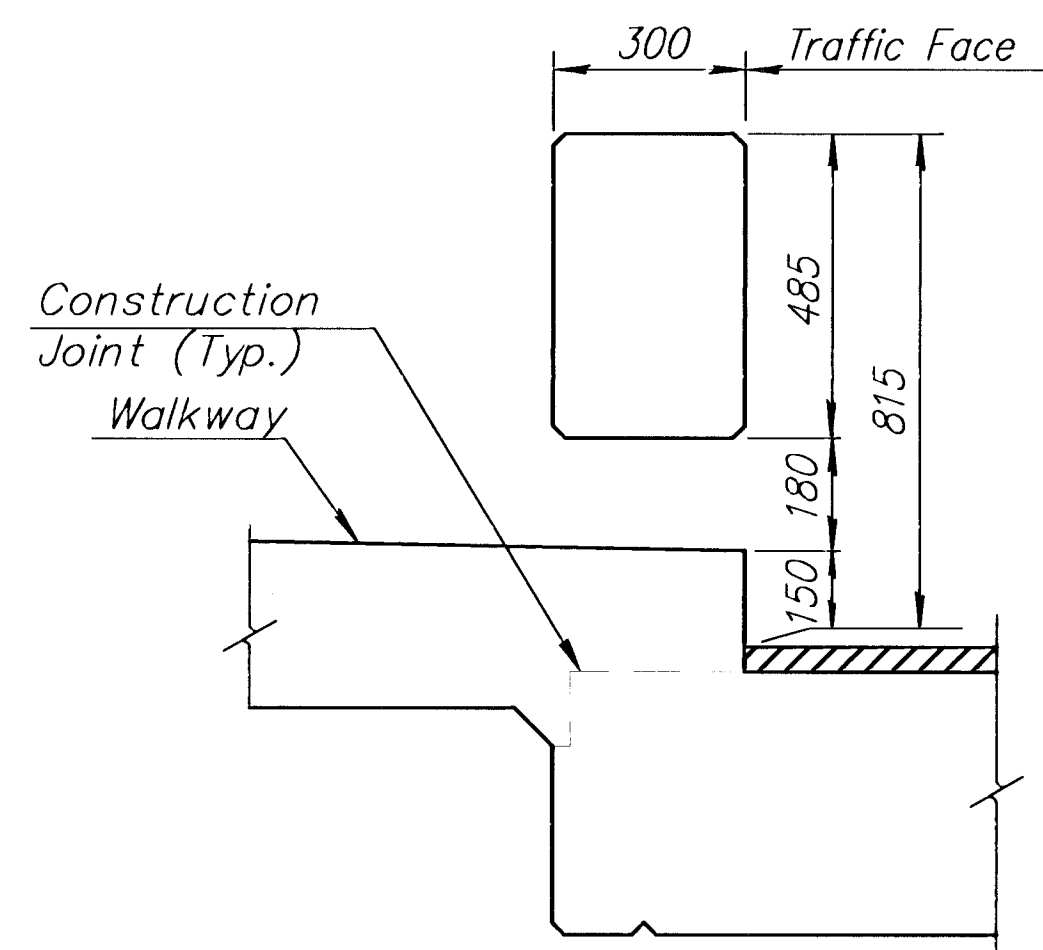
TYPICAL SECTION BETWEEN POSTS
