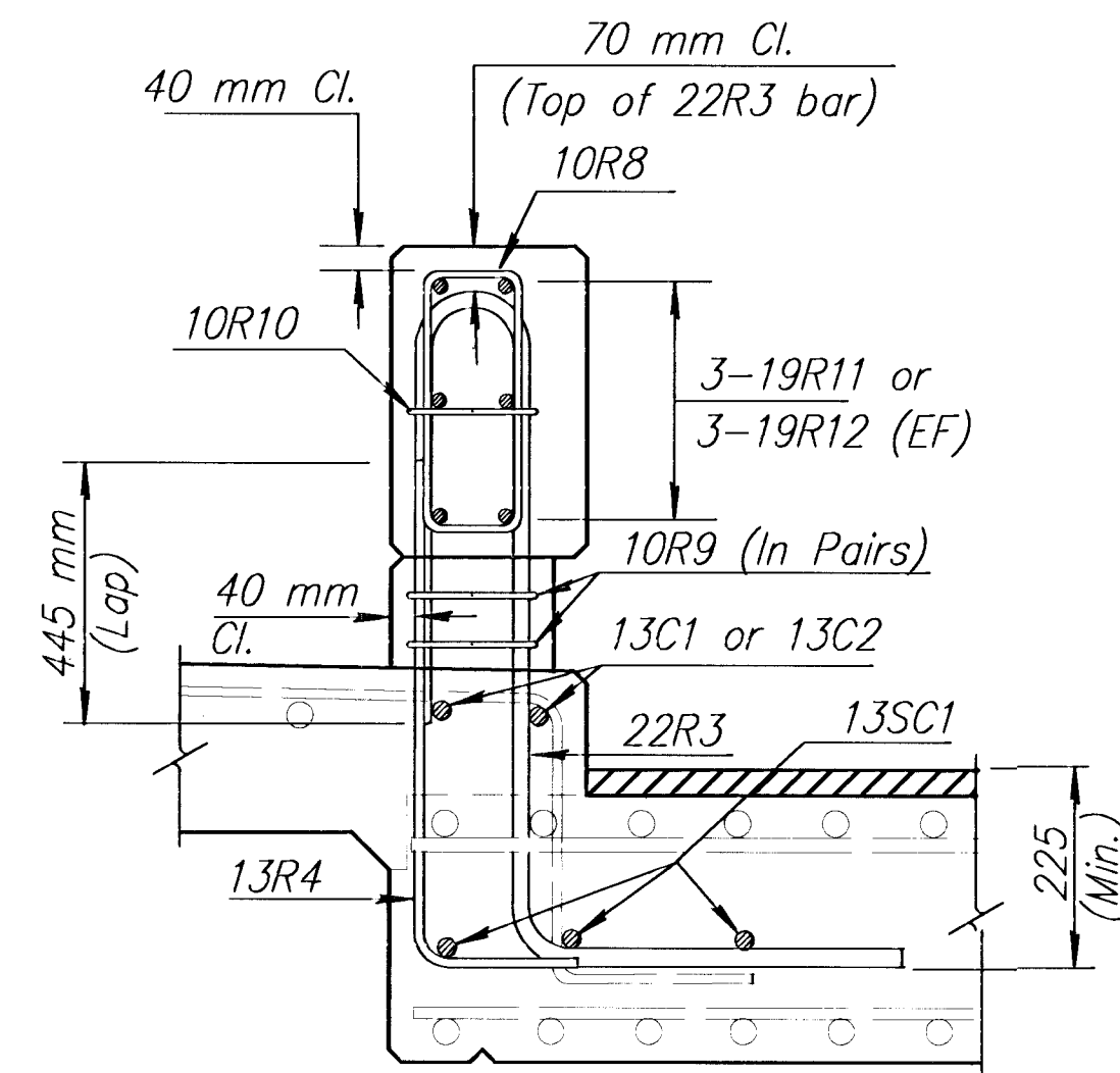
TYPICAL SECTION INTERIOR POST
