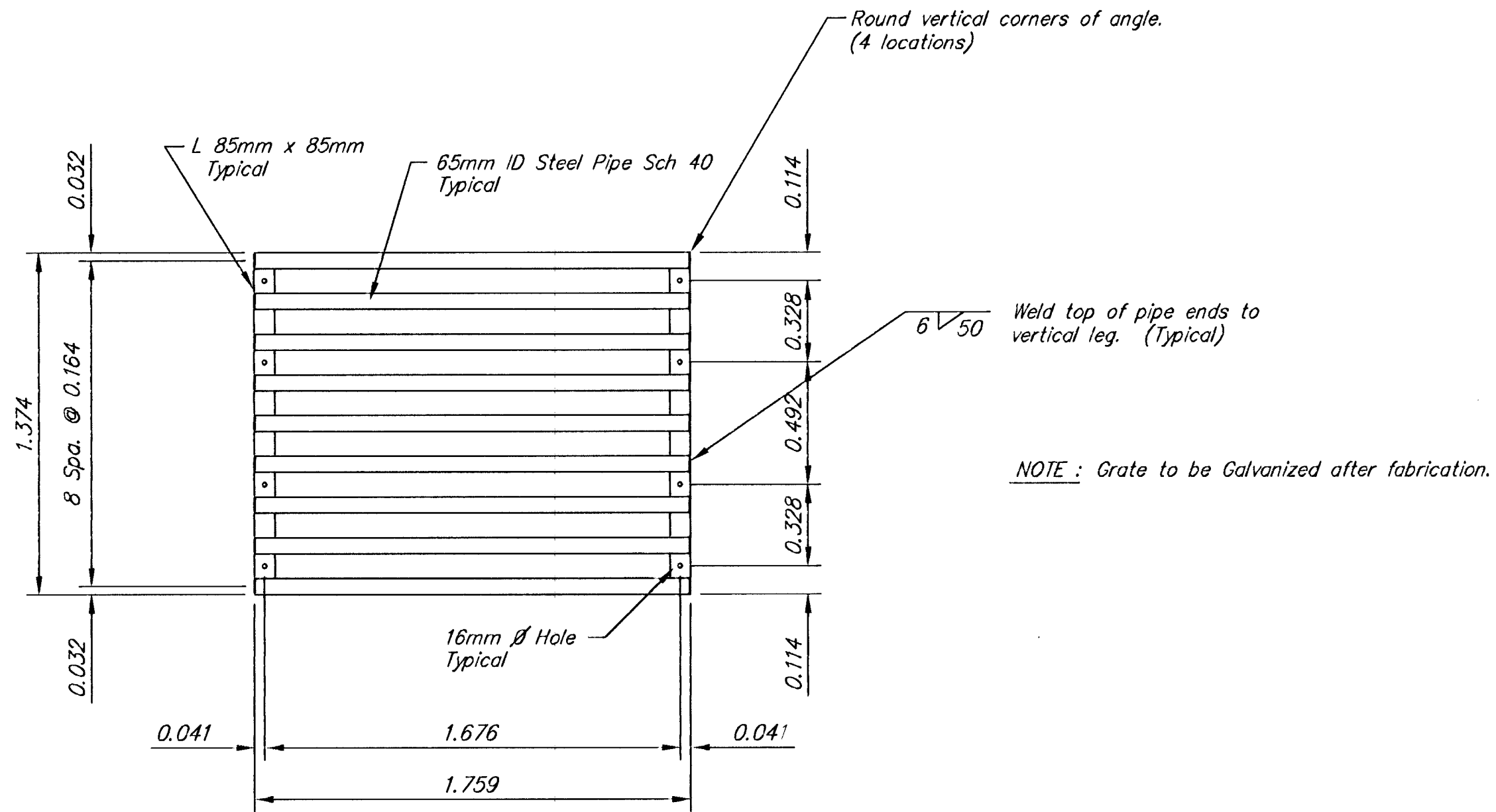
PIPE GRATE DETAILS
