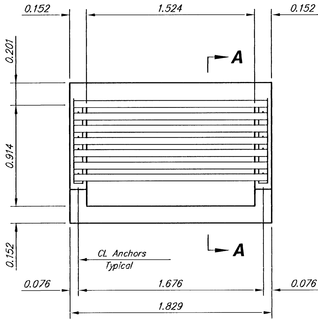
END VIEW
