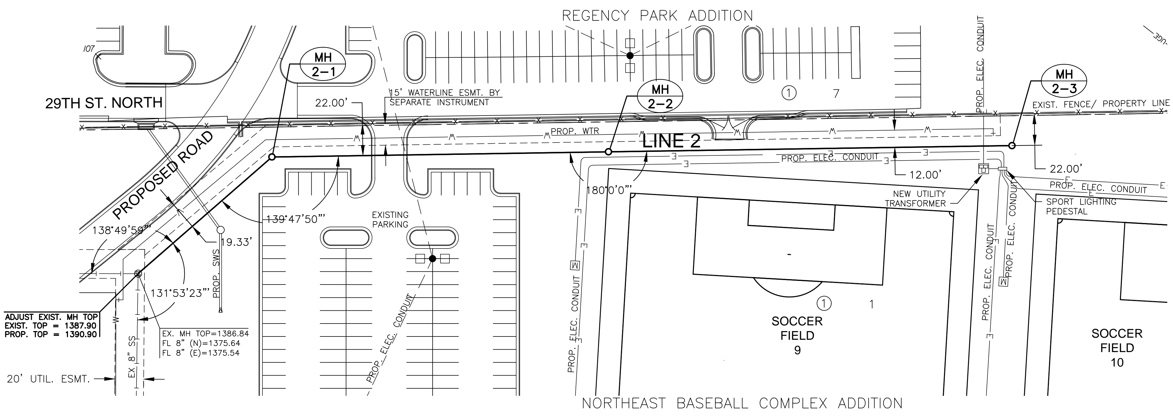
PLAN SAN LINE 2 PROFILE SAN LINE 2
