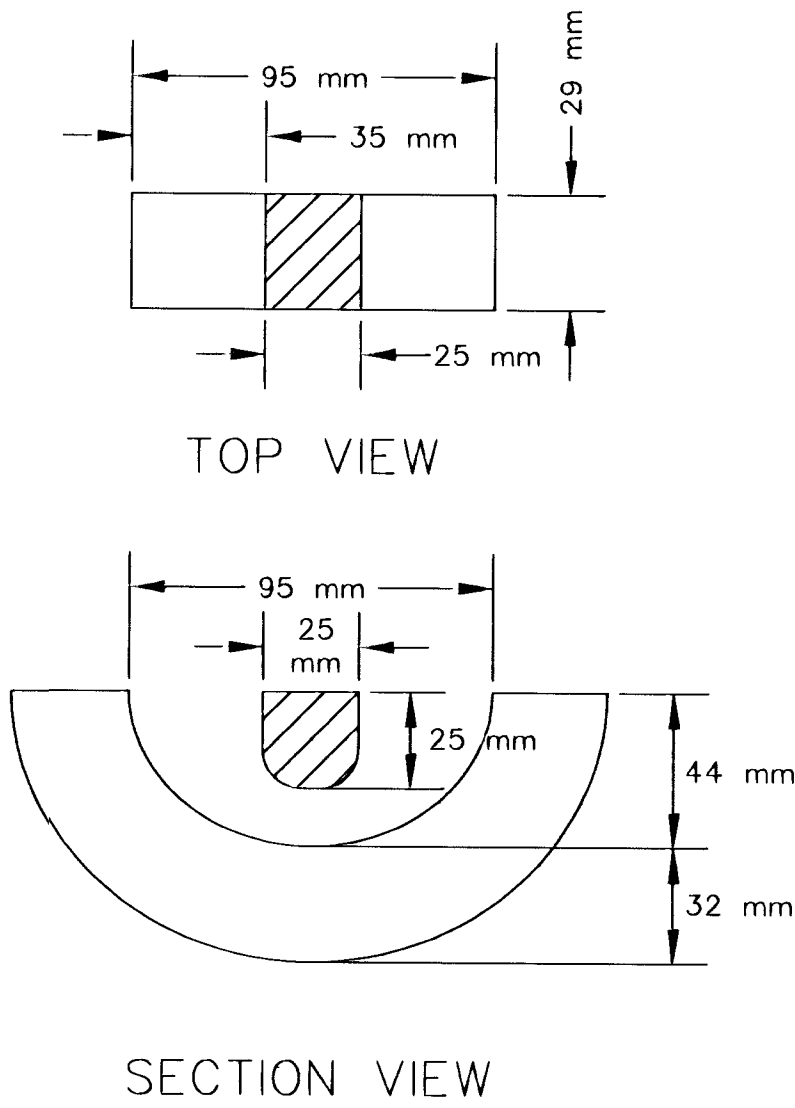
PICKHOLE DETAIL
