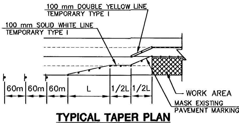
TYPICAL TAPER PLAN
