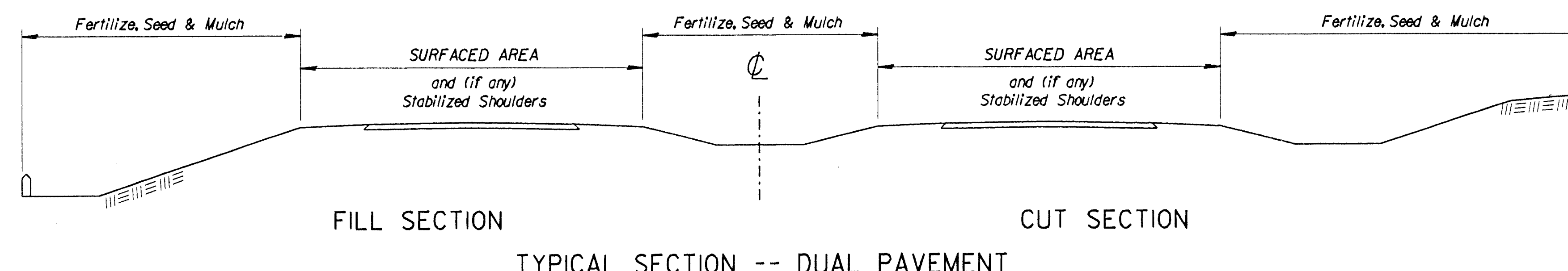
TYPICAL SECTION -- DUAL PAVEMENT
