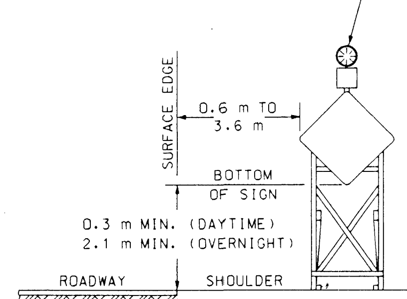
HEIGHT AND LATERAL DIMENSIONS FOR SIGNS MOUNTED ON SKIDS OR OTHER MOVABLE MOUNTS
