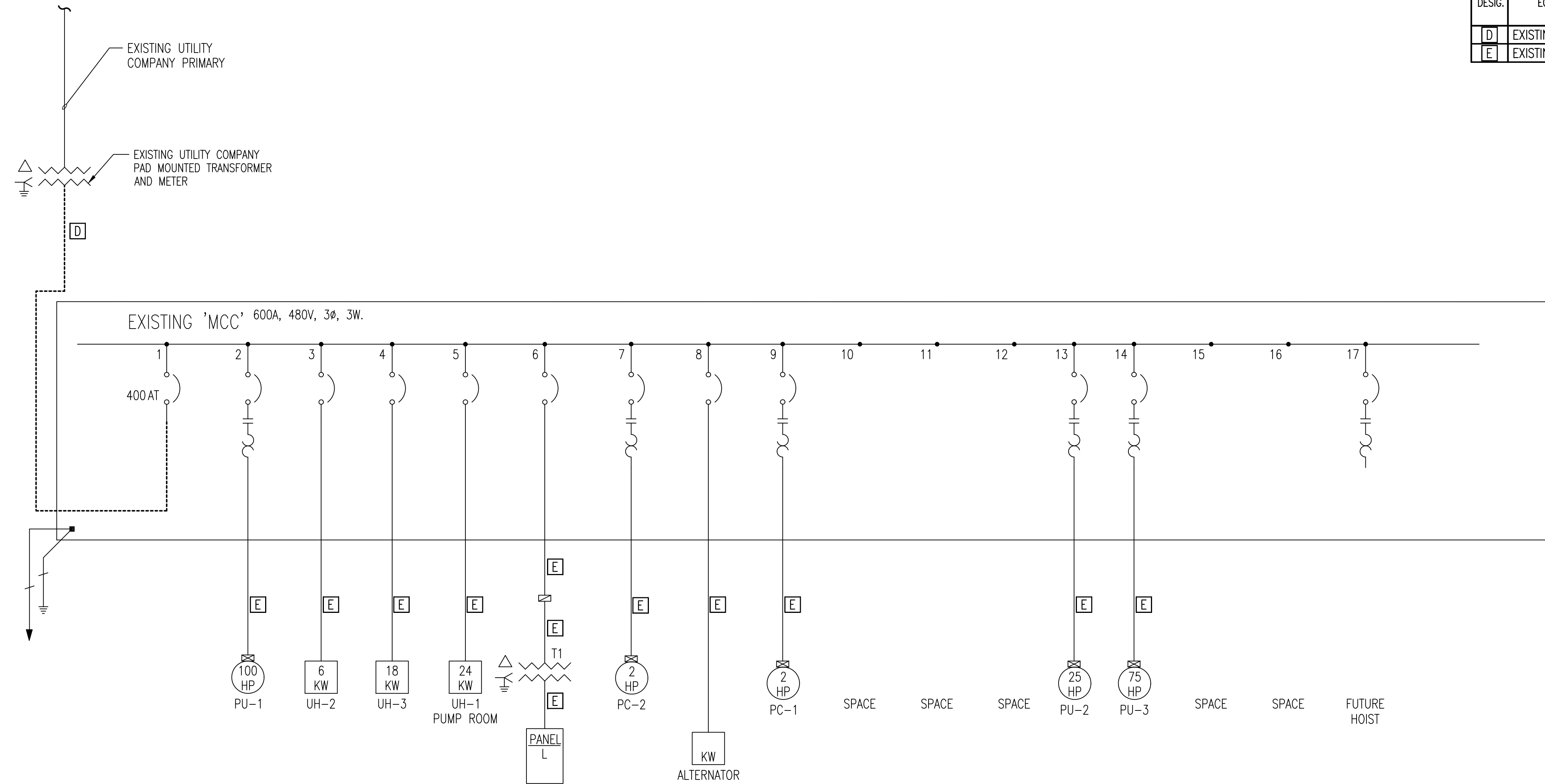
1 ELECTRICAL ONE-LINE DIAGRAM - DEMOLITION NO SCALE
