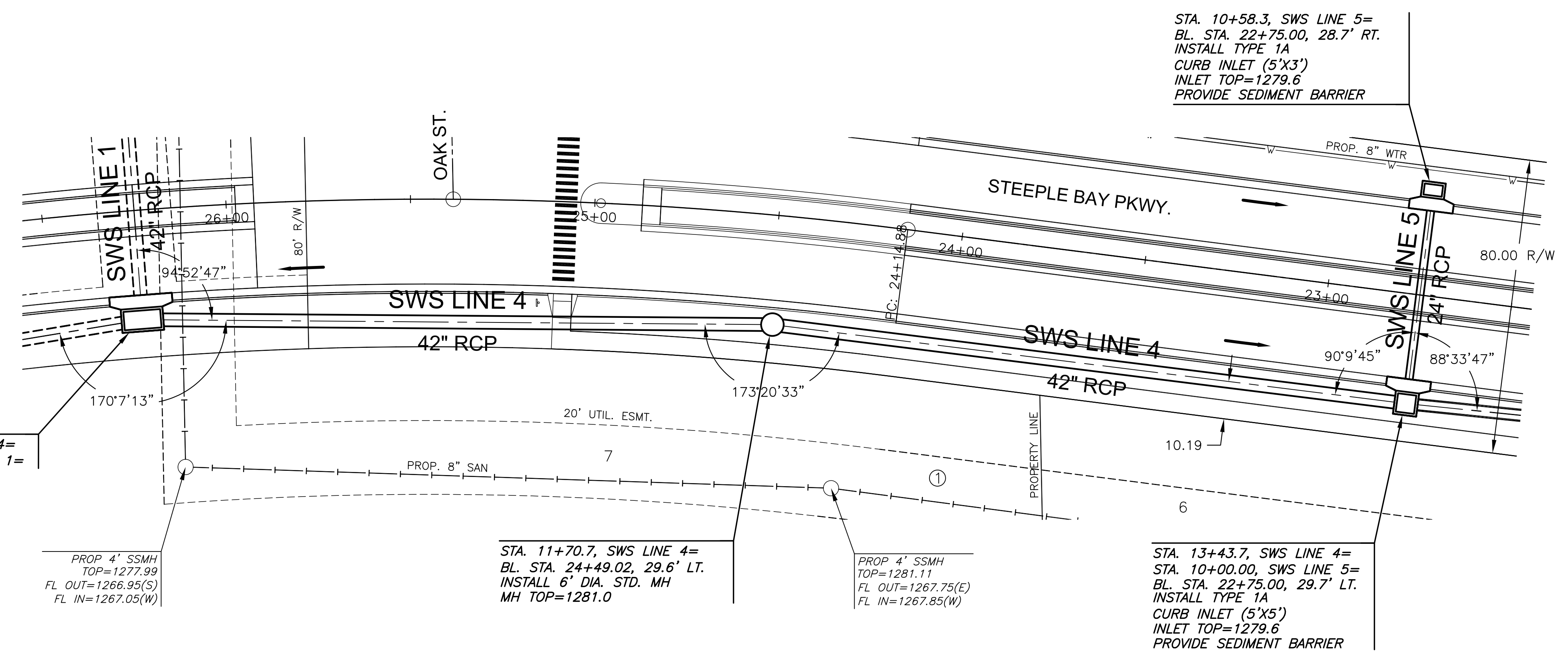
PLAN SWS LINE 4 PROFILE SWS LINE 4
