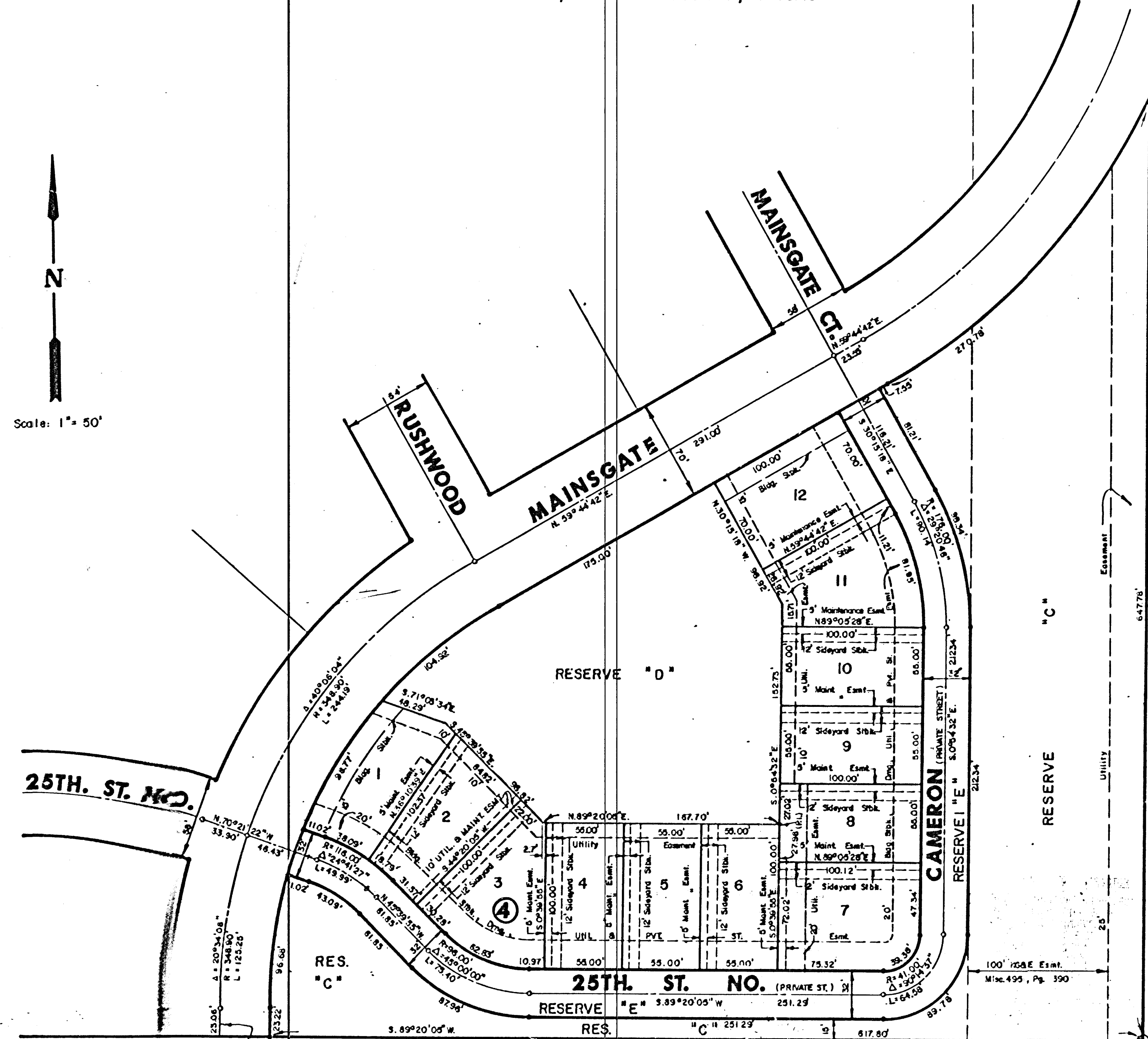
DETAIL "A"
