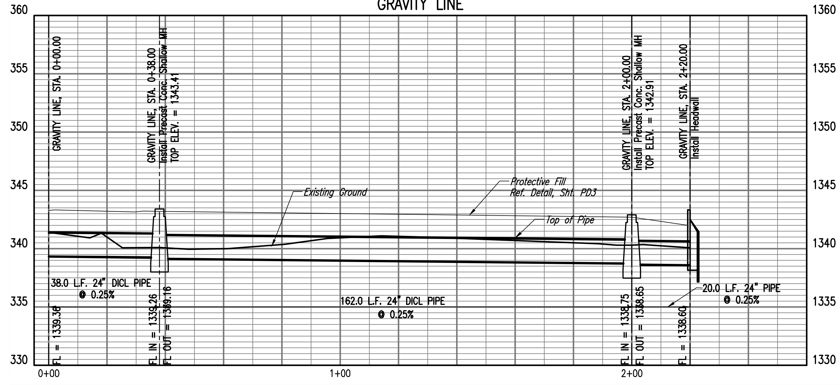
GRAVITY LINE
